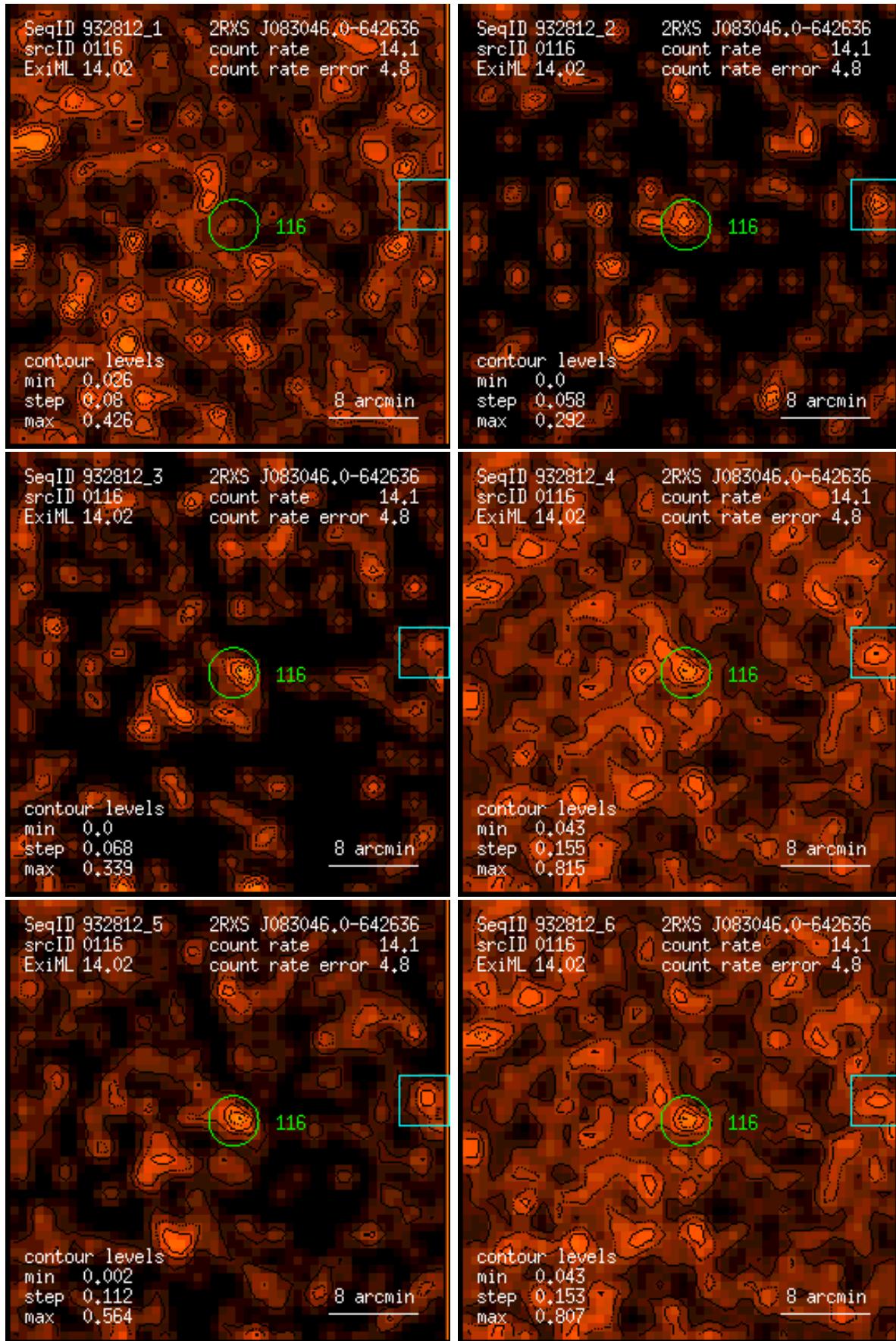
Figure 116: RASS 932812: detection 0116: band rate images, Gaussian filter: (1) PSPC channels 11 – 41, (2) 52 – 90, (3) 91 – 201, (4) 11 – 235, (5) 52 – 201, (6) 11 – 201. Broad band rates in counts/ks. Band rate contour levels in counts/ks/arcmin 2 .
