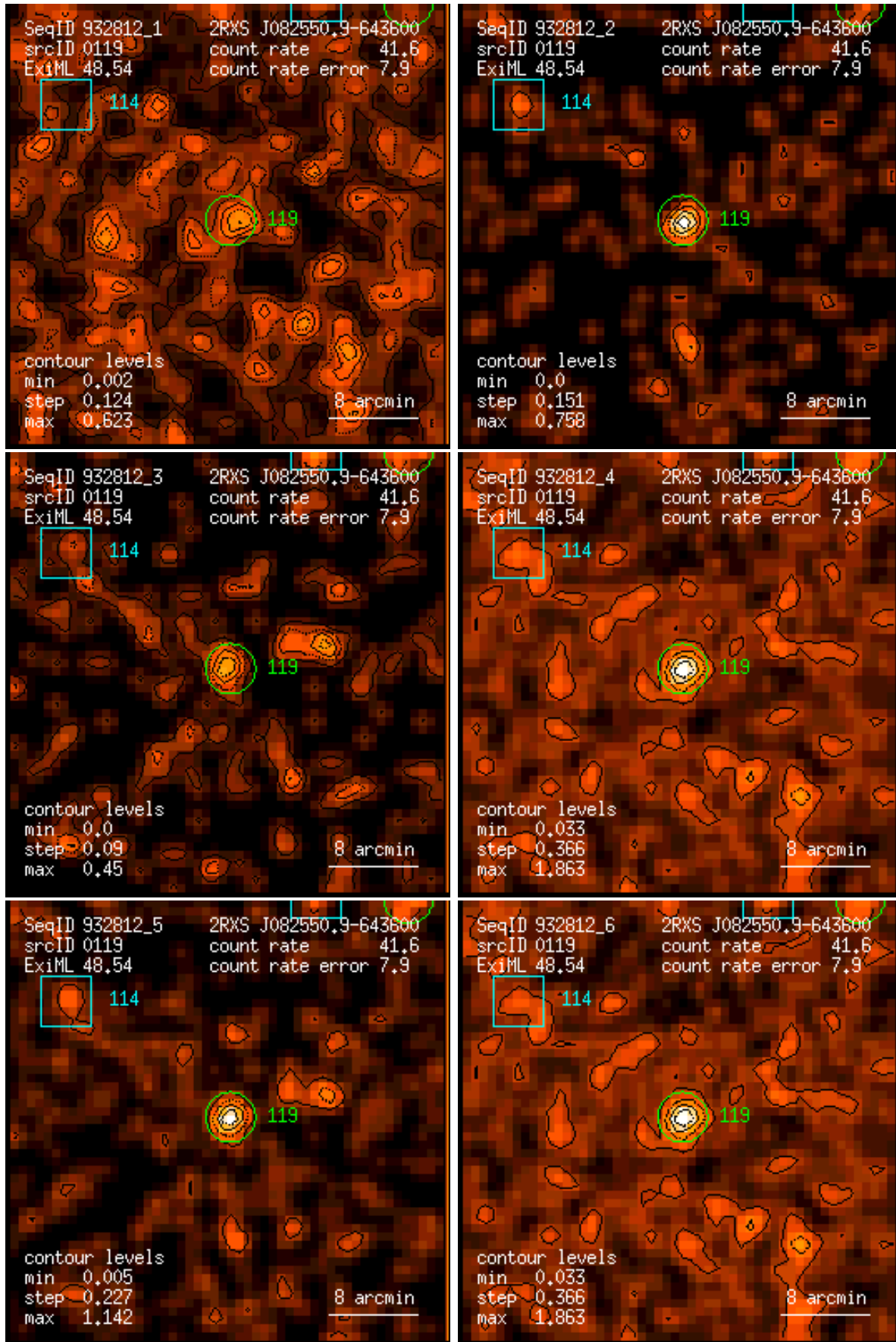
Figure 119: RASS 932812: detection 0119: band rate images, Gaussian filter: (1) PSPC channels 11 – 41, (2) 52 – 90, (3) 91 – 201, (4) 11 – 235, (5) 52 – 201, (6) 11 – 201. Broad band rates in counts/ks. Band rate contour levels in counts/ks/arcmin 2 .
