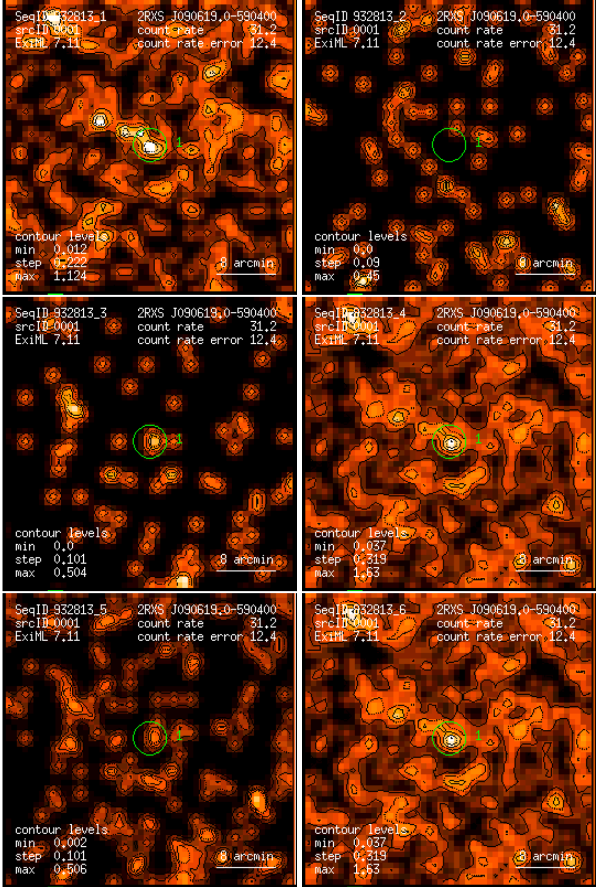
Figure 1: RASS 932813: detection 0001: band rate images, Gaussian filter: (1) PSPC channels 11 – 41, (2) 52 – 90, (3) 91 – 201, (4) 11 – 235, (5) 52 – 201, (6) 11 – 201. Broad band rates in counts/ks. Band rate contour levels in counts/ks/arcmin 2 .
