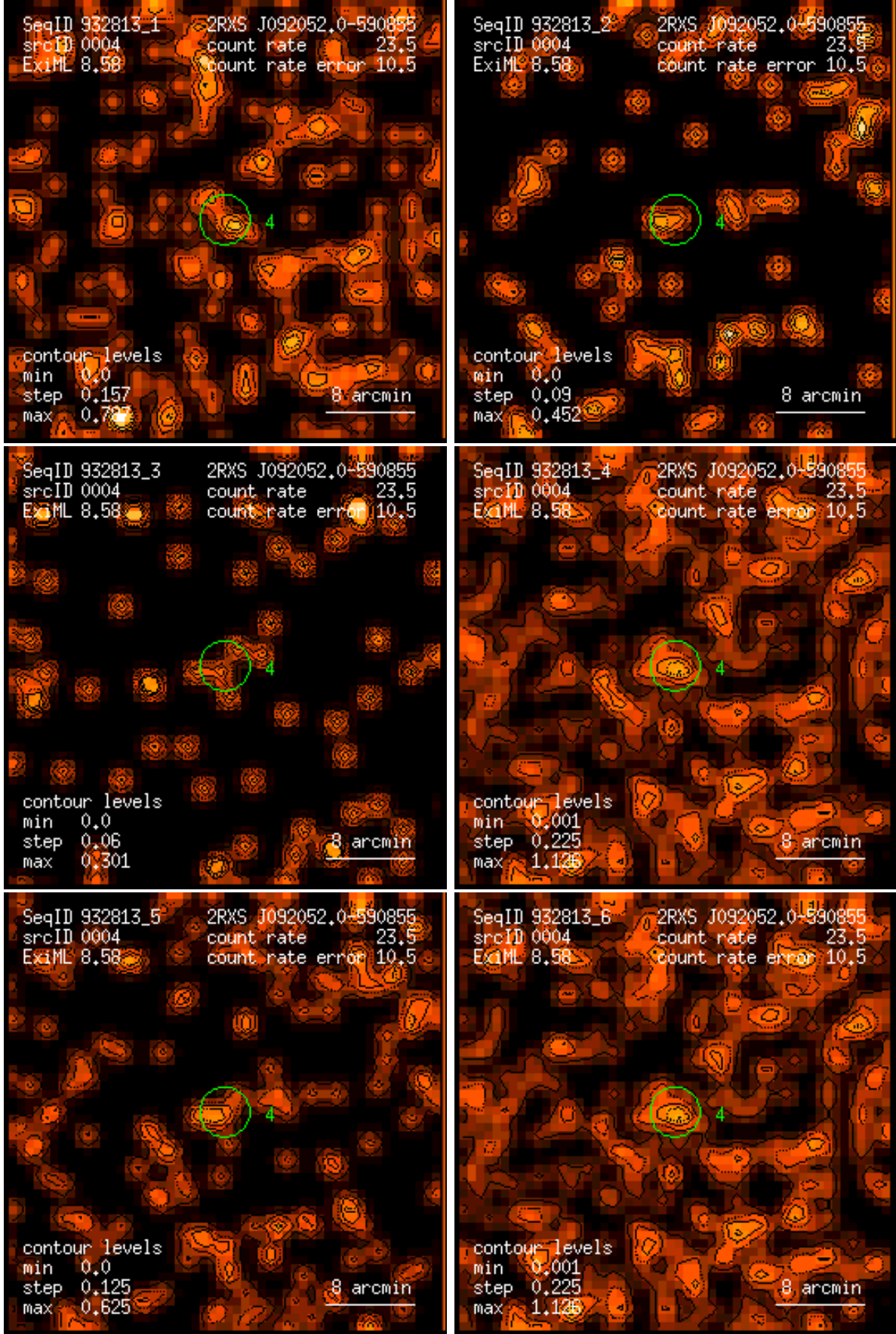
Figure 4: RASS 932813: detection 0004: band rate images, Gaussian filter: (1) PSPC channels 11 – 41, (2) 52 – 90, (3) 91 – 201, (4) 11 – 235, (5) 52 – 201, (6) 11 – 201. Broad band rates in counts/ks. Band rate contour levels in counts/ks/arcmin 2 .
