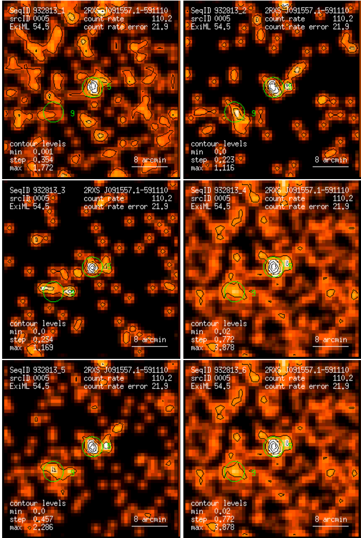
Figure 5: RASS 932813: detection 0005: band rate images, Gaussian filter: (1) PSPC channels 11 – 41, (2) 52 – 90, (3) 91 – 201, (4) 11 – 235, (5) 52 – 201, (6) 11 – 201. Broad band rates in counts/ks. Band rate contour levels in counts/ks/arcmin 2 .
