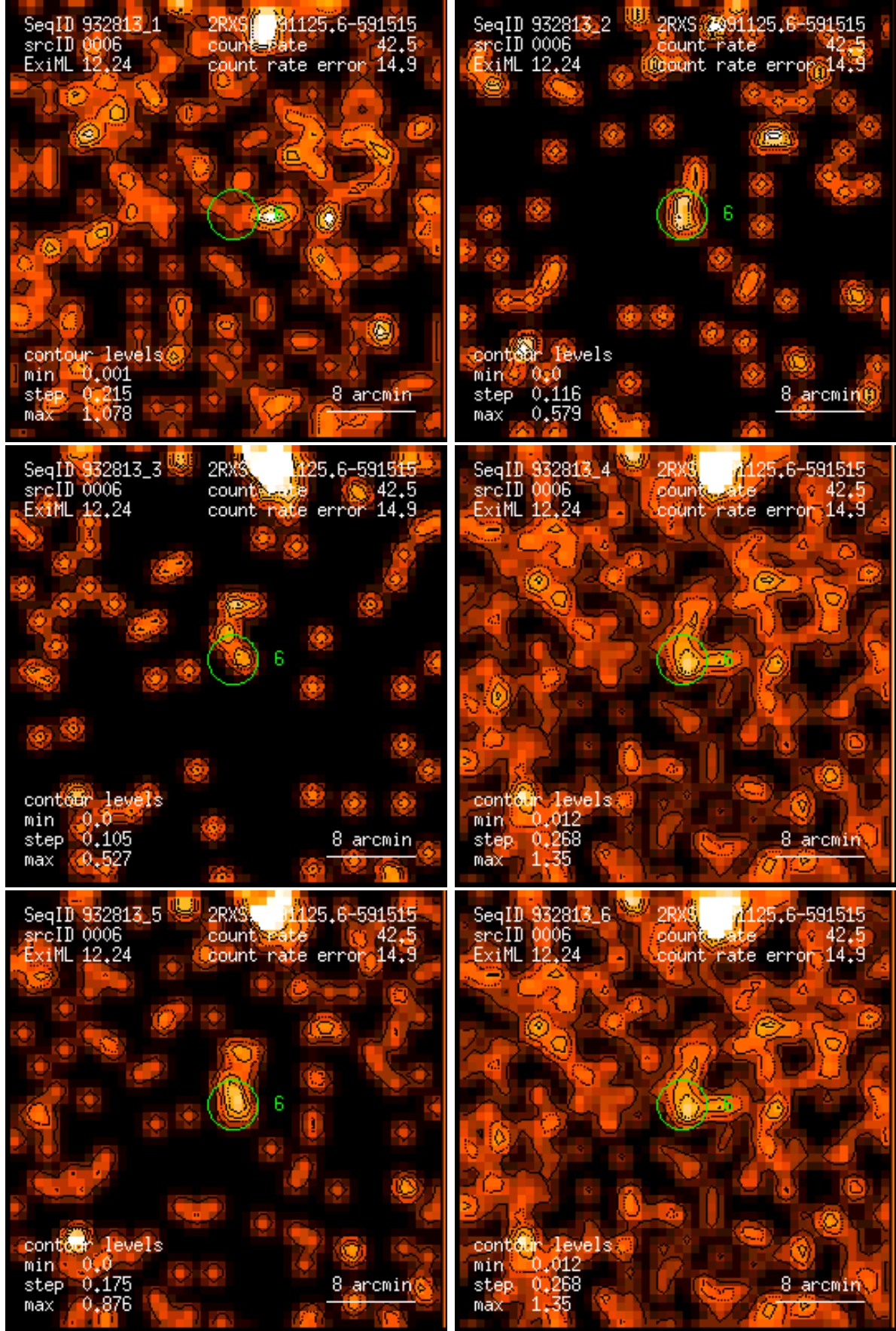
Figure 6: RASS 932813: detection 0006: band rate images, Gaussian filter: (1) PSPC channels 11 – 41, (2) 52 – 90, (3) 91 – 201, (4) 11 – 235, (5) 52 – 201, (6) 11 – 201. Broad band rates in counts/ks. Band rate contour levels in counts/ks/arcmin 2 .
