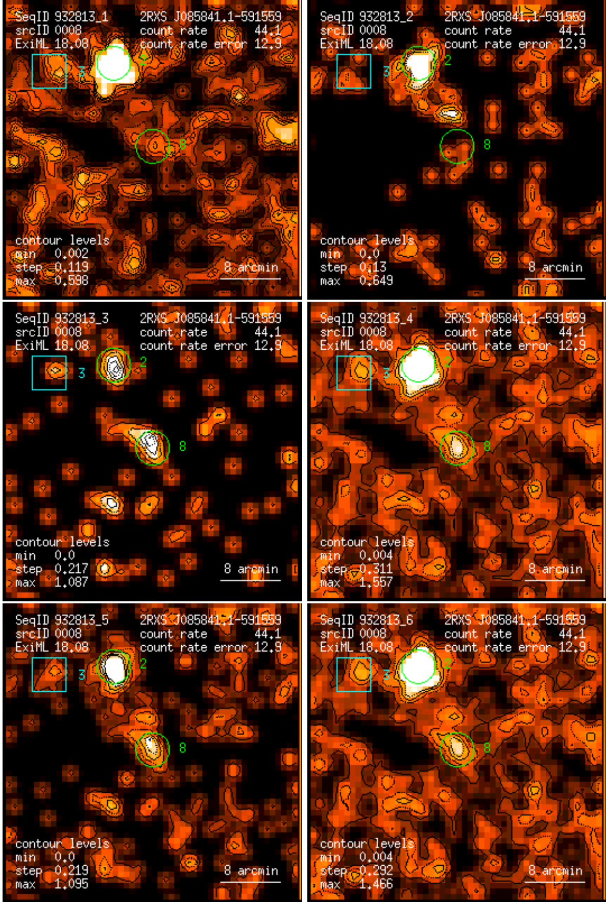
Figure 8: RASS 932813: detection 0008: band rate images, Gaussian filter: (1) PSPC channels 11 – 41, (2) 52 – 90, (3) 91 – 201, (4) 11 – 235, (5) 52 – 201, (6) 11 – 201. Broad band rates in counts/ks. Band rate contour levels in counts/ks/arcmin 2 .
