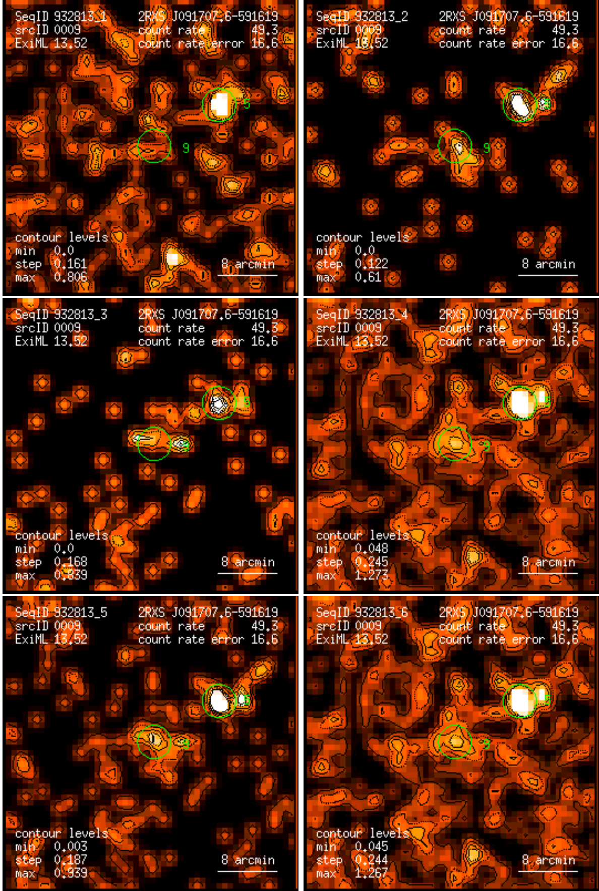
Figure 9: RASS 932813: detection 0009: band rate images, Gaussian filter: (1) PSPC channels 11 – 41, (2) 52 – 90, (3) 91 – 201, (4) 11 – 235, (5) 52 – 201, (6) 11 – 201. Broad band rates in counts/ks. Band rate contour levels in counts/ks/arcmin 2 .
