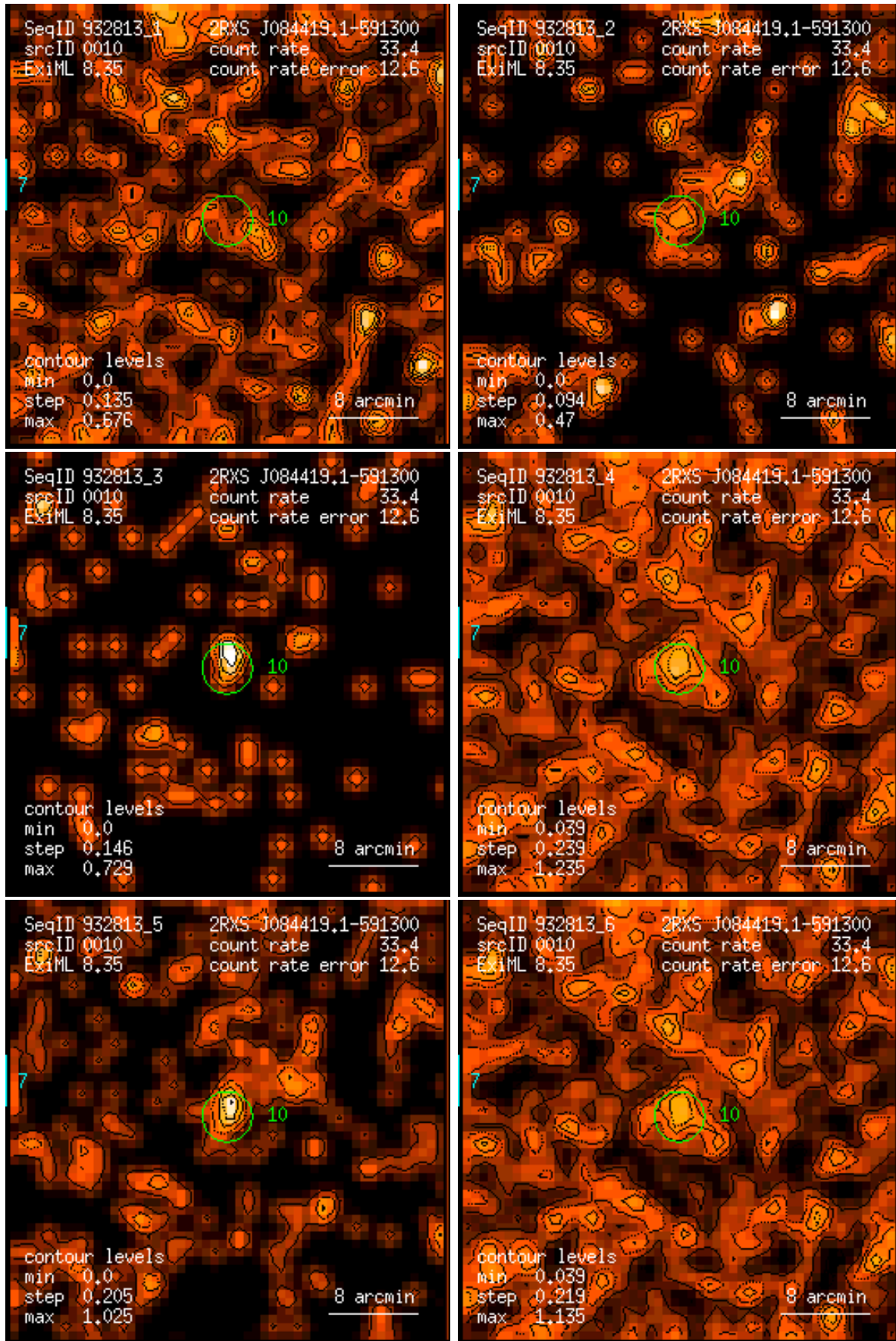
Figure 10: RASS 932813: detection 0010: band rate images, Gaussian filter: (1) PSPC channels 11 – 41, (2) 52 – 90, (3) 91 – 201, (4) 11 – 235, (5) 52 – 201, (6) 11 – 201. Broad band rates in counts/ks. Band rate contour levels in counts/ks/arcmin 2 .
