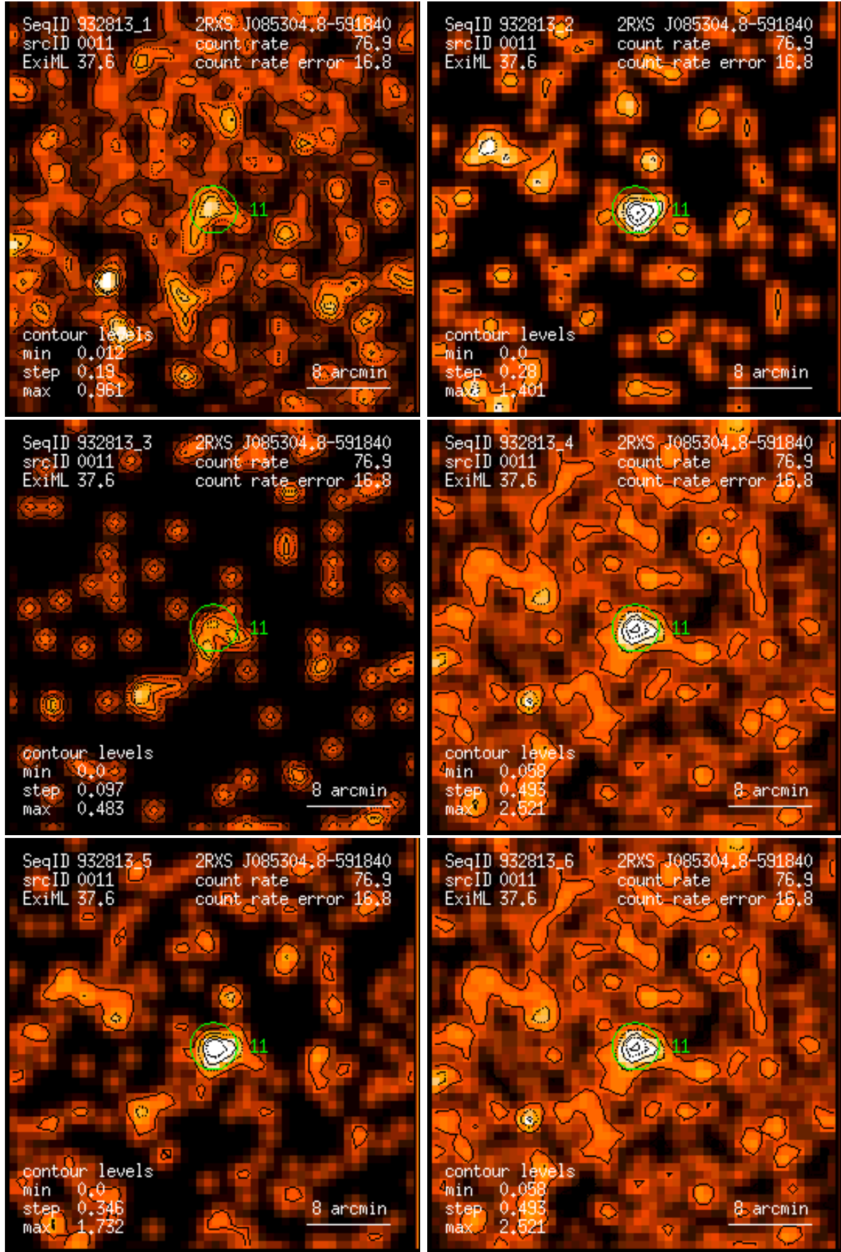
Figure 11: RASS 932813: detection 0011: band rate images, Gaussian filter: (1) PSPC channels 11 – 41, (2) 52 – 90, (3) 91 – 201, (4) 11 – 235, (5) 52 – 201, (6) 11 – 201. Broad band rates in counts/ks. Band rate contour levels in counts/ks/arcmin 2 .
