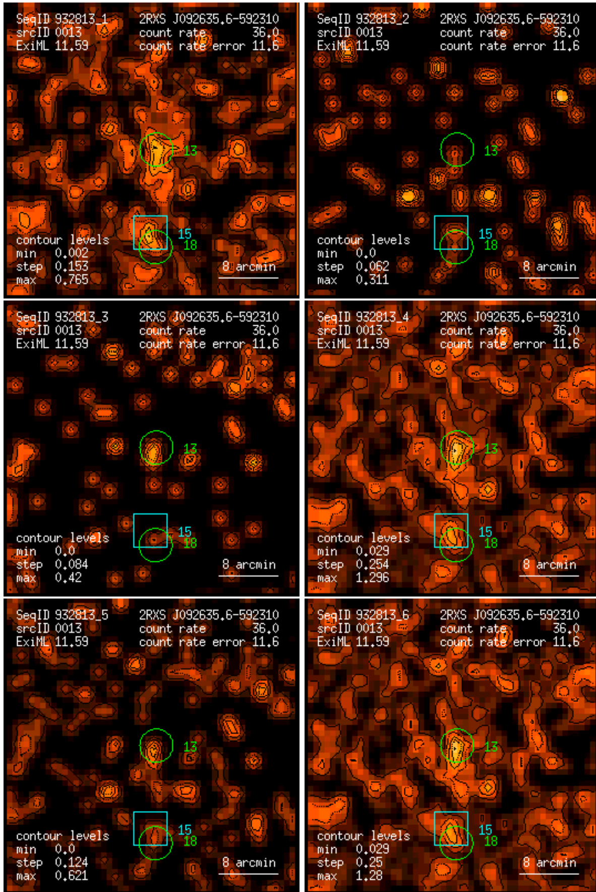
Figure 13: RASS 932813: detection 0013: band rate images, Gaussian filter: (1) PSPC channels 11 – 41, (2) 52 – 90, (3) 91 – 201, (4) 11 – 235, (5) 52 – 201, (6) 11 – 201. Broad band rates in counts/ks. Band rate contour levels in counts/ks/arcmin 2 .
