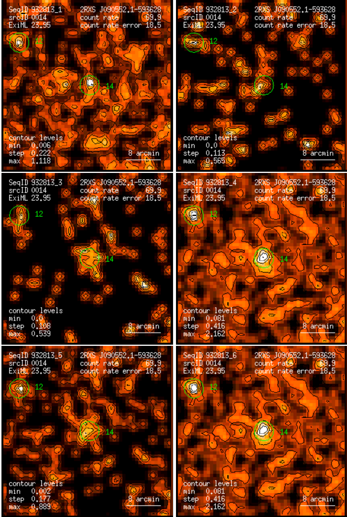
Figure 14: RASS 932813: detection 0014: band rate images, Gaussian filter: (1) PSPC channels 11 – 41, (2) 52 – 90, (3) 91 – 201, (4) 11 – 235, (5) 52 – 201, (6) 11 – 201. Broad band rates in counts/ks. Band rate contour levels in counts/ks/arcmin 2 .
