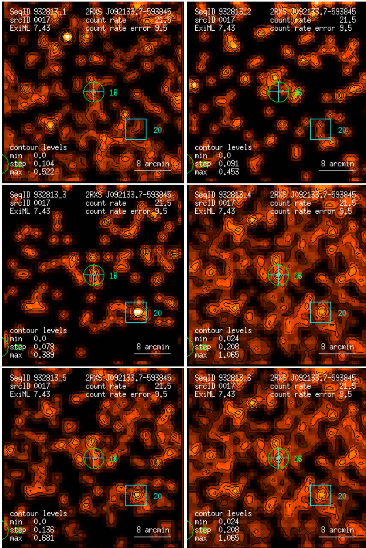
Figure 17: RASS 932813: detection 0017: band rate images, Gaussian filter: (1) PSPC channels 11 – 41, (2) 52 – 90, (3) 91 – 201, (4) 11 – 235, (5) 52 – 201, (6) 11 – 201. Broad band rates in counts/ks. Band rate contour levels in counts/ks/arcmin 2 .
