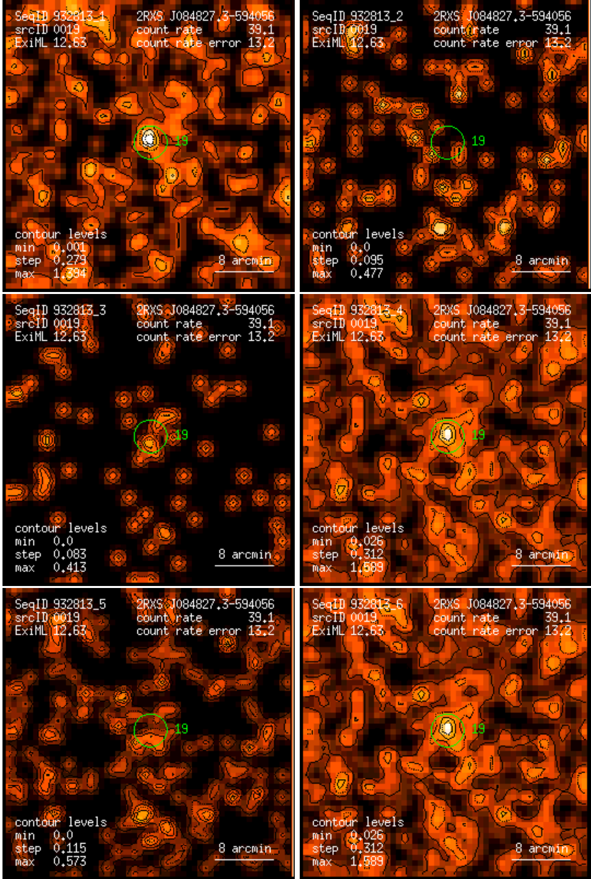
Figure 19: RASS 932813: detection 0019: band rate images, Gaussian filter: (1) PSPC channels 11 – 41, (2) 52 – 90, (3) 91 – 201, (4) 11 – 235, (5) 52 – 201, (6) 11 – 201. Broad band rates in counts/ks. Band rate contour levels in counts/ks/arcmin 2 .
