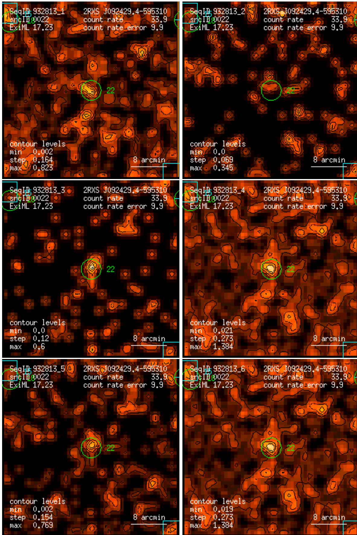
Figure 22: RASS 932813: detection 0022: band rate images, Gaussian filter: (1) PSPC channels 11 – 41, (2) 52 – 90, (3) 91 – 201, (4) 11 – 235, (5) 52 – 201, (6) 11 – 201. Broad band rates in counts/ks. Band rate contour levels in counts/ks/arcmin 2 .
