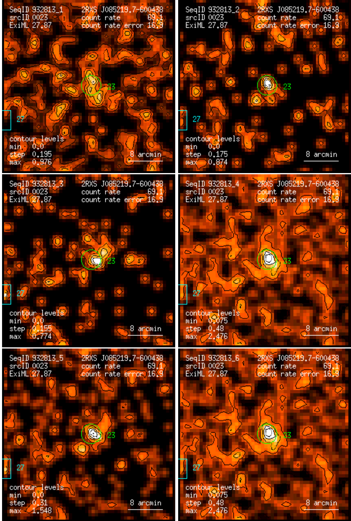
Figure 23: RASS 932813: detection 0023: band rate images, Gaussian filter: (1) PSPC channels 11 – 41, (2) 52 – 90, (3) 91 – 201, (4) 11 – 235, (5) 52 – 201, (6) 11 – 201. Broad band rates in counts/ks. Band rate contour levels in counts/ks/arcmin 2 .
