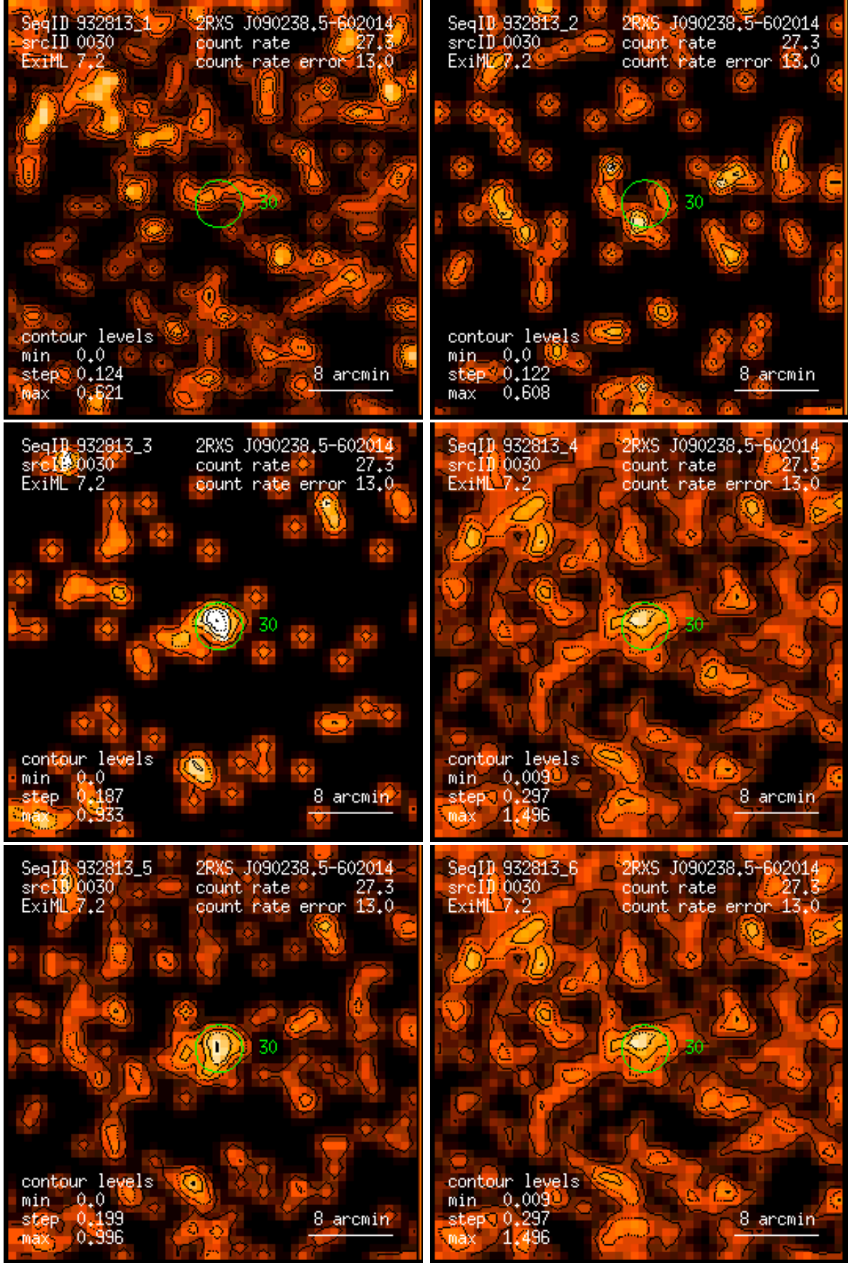
Figure 30: RASS 932813: detection 0030: band rate images, Gaussian filter: (1) PSPC channels 11 – 41, (2) 52 – 90, (3) 91 – 201, (4) 11 – 235, (5) 52 – 201, (6) 11 – 201. Broad band rates in counts/ks. Band rate contour levels in counts/ks/arcmin 2 .
