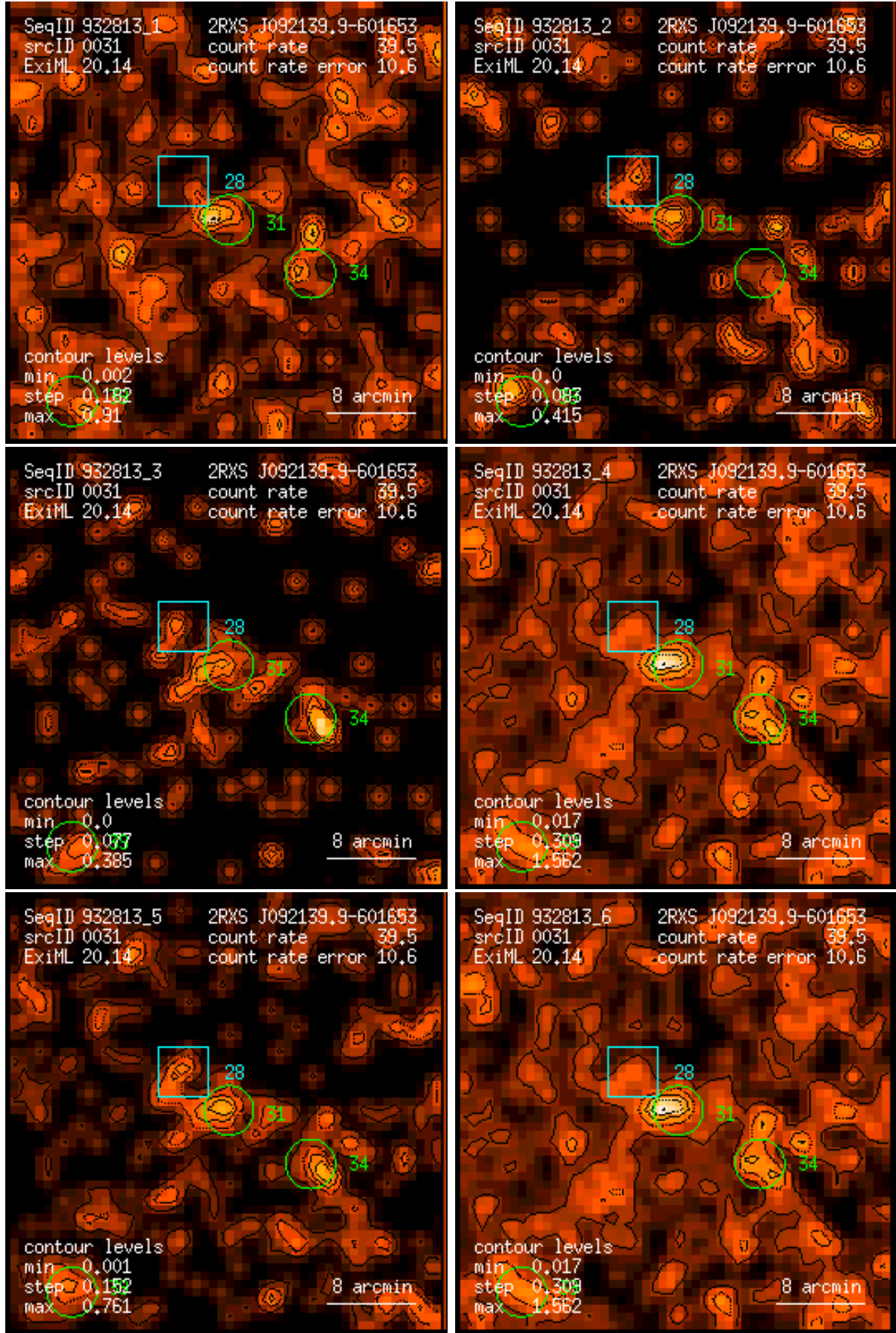
Figure 31: RASS 932813: detection 0031: band rate images, Gaussian filter: (1) PSPC channels 11 – 41, (2) 52 – 90, (3) 91 – 201, (4) 11 – 235, (5) 52 – 201, (6) 11 – 201. Broad band rates in counts/ks. Band rate contour levels in counts/ks/arcmin 2 .
