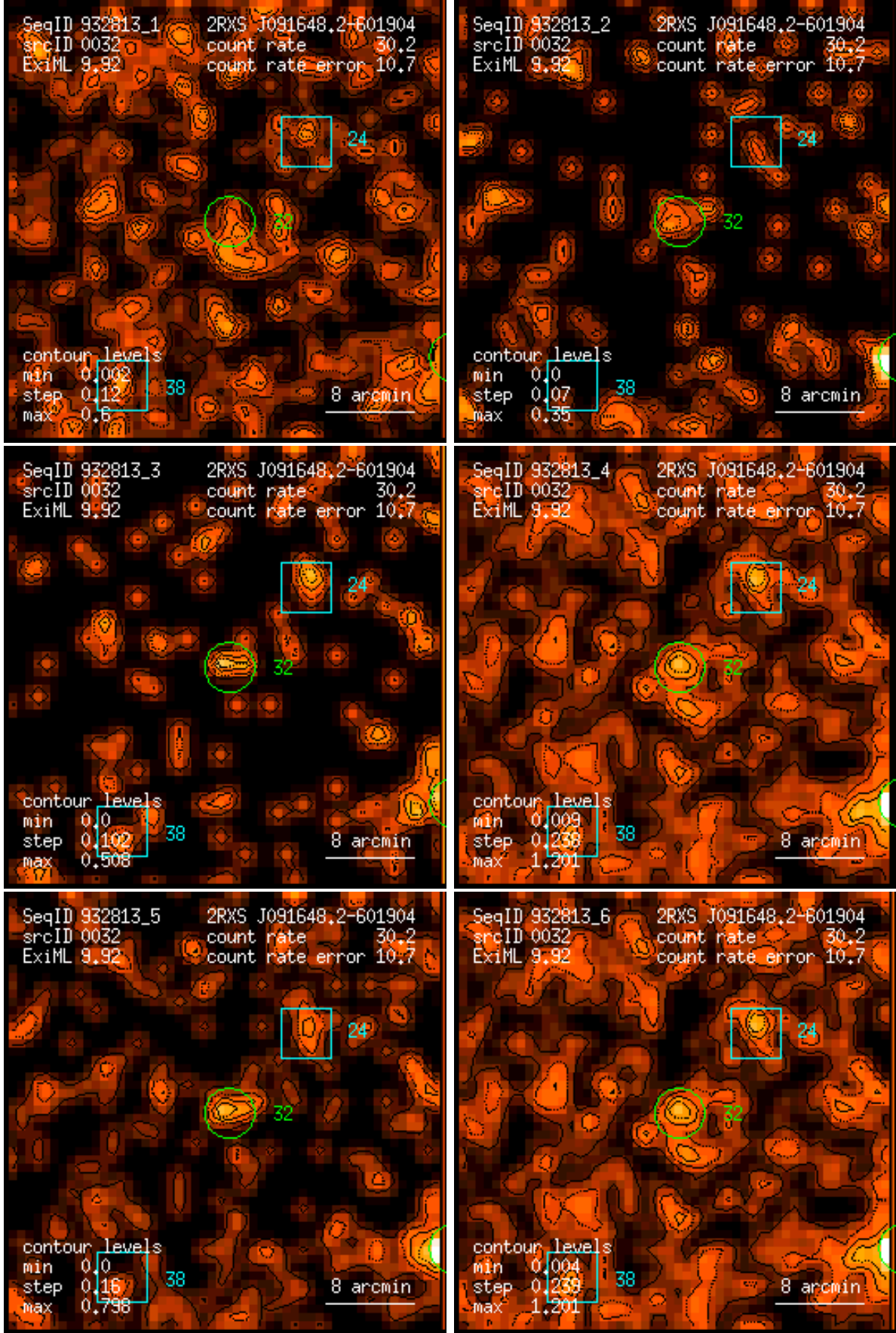
Figure 32: RASS 932813: detection 0032: band rate images, Gaussian filter: (1) PSPC channels 11 – 41, (2) 52 – 90, (3) 91 – 201, (4) 11 – 235, (5) 52 – 201, (6) 11 – 201. Broad band rates in counts/ks. Band rate contour levels in counts/ks/arcmin 2 .
