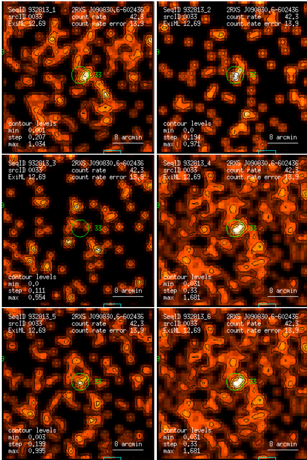
Figure 33: RASS 932813: detection 0033: band rate images, Gaussian filter: (1) PSPC channels 11 – 41, (2) 52 – 90, (3) 91 – 201, (4) 11 – 235, (5) 52 – 201, (6) 11 – 201. Broad band rates in counts/ks. Band rate contour levels in counts/ks/arcmin 2 .
