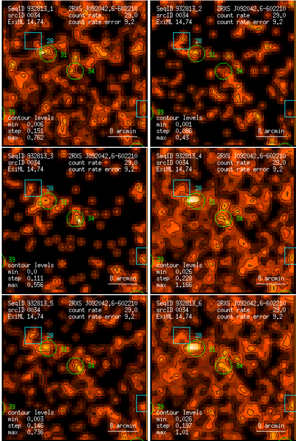
Figure 34: RASS 932813: detection 0034: band rate images, Gaussian filter: (1) PSPC channels 11 – 41, (2) 52 – 90, (3) 91 – 201, (4) 11 – 235, (5) 52 – 201, (6) 11 – 201. Broad band rates in counts/ks. Band rate contour levels in counts/ks/arcmin 2 .
