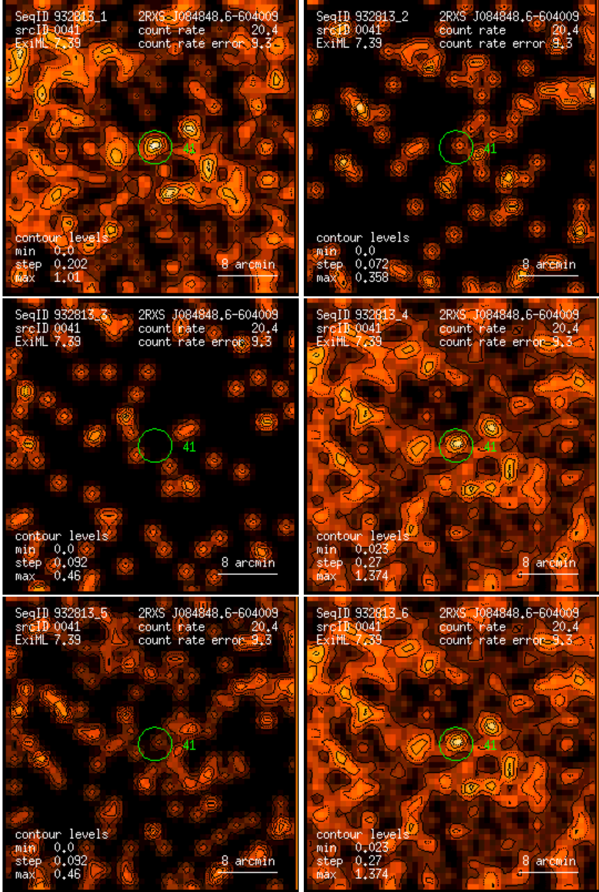
Figure 41: RASS 932813: detection 0041: band rate images, Gaussian filter: (1) PSPC channels 11 – 41, (2) 52 – 90, (3) 91 – 201, (4) 11 – 235, (5) 52 – 201, (6) 11 – 201. Broad band rates in counts/ks. Band rate contour levels in counts/ks/arcmin 2 .
