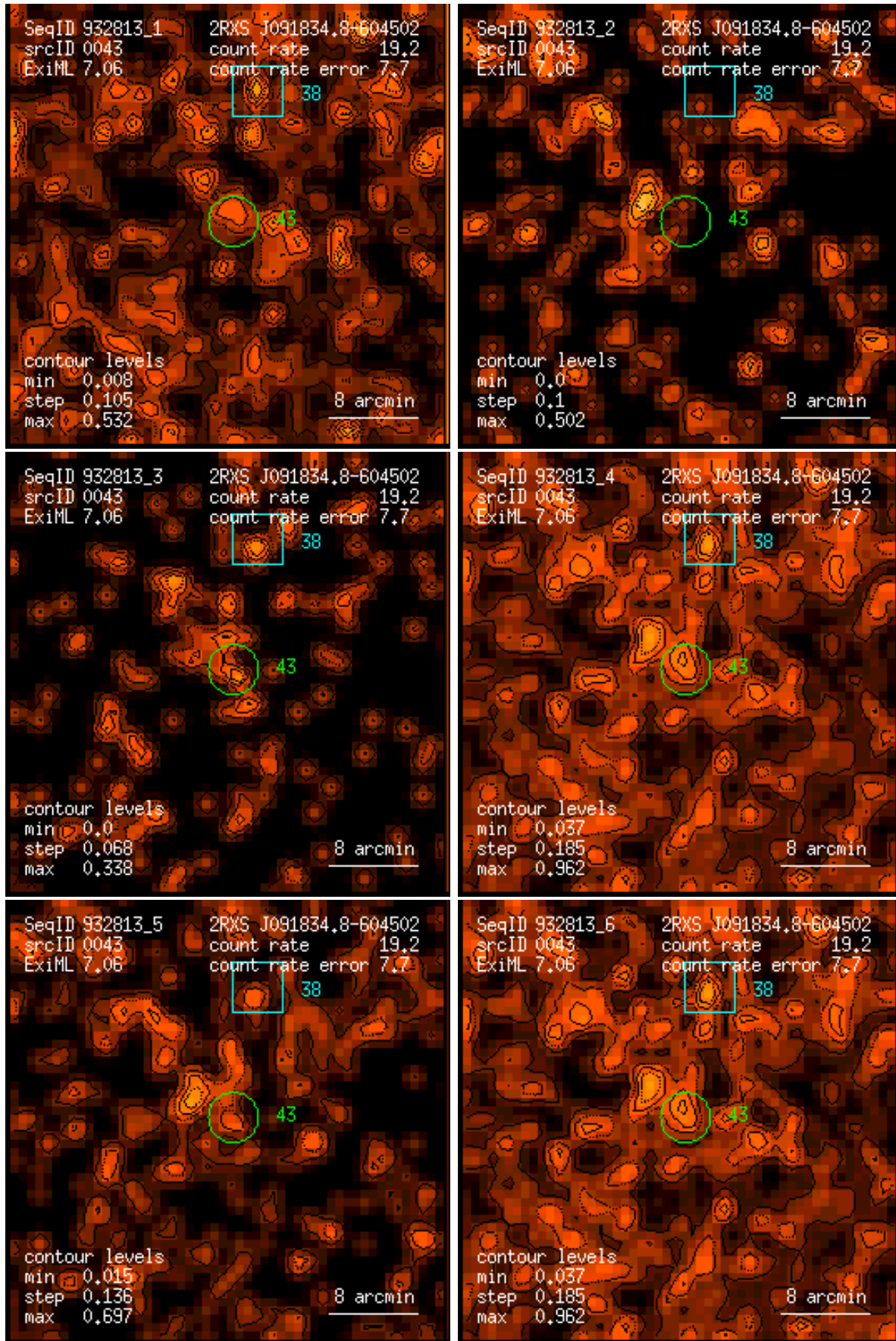
Figure 43: RASS 932813: detection 0043: band rate images, Gaussian filter: (1) PSPC channels 11 – 41, (2) 52 – 90, (3) 91 – 201, (4) 11 – 235, (5) 52 – 201, (6) 11 – 201. Broad band rates in counts/ks. Band rate contour levels in counts/ks/arcmin 2 .
