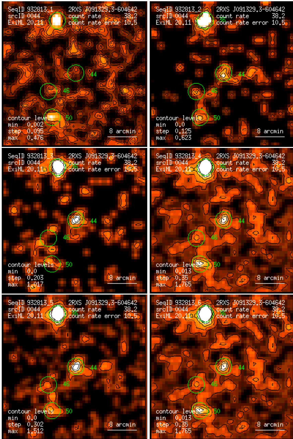
Figure 44: RASS 932813: detection 0044: band rate images, Gaussian filter: (1) PSPC channels 11 – 41, (2) 52 – 90, (3) 91 – 201, (4) 11 – 235, (5) 52 – 201, (6) 11 – 201. Broad band rates in counts/ks. Band rate contour levels in counts/ks/arcmin 2 .
