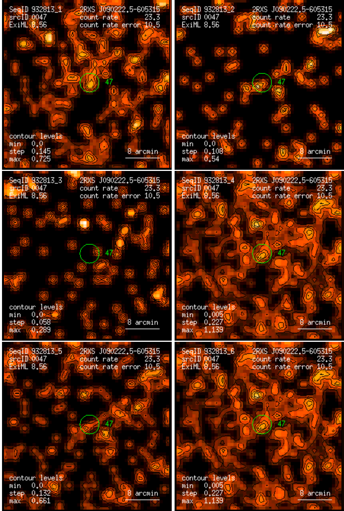
Figure 47: RASS 932813: detection 0047: band rate images, Gaussian filter: (1) PSPC channels 11 – 41, (2) 52 – 90, (3) 91 – 201, (4) 11 – 235, (5) 52 – 201, (6) 11 – 201. Broad band rates in counts/ks. Band rate contour levels in counts/ks/arcmin 2 .
