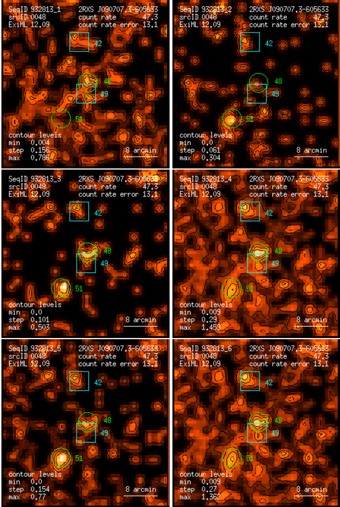
Figure 48: RASS 932813: detection 0048: band rate images, Gaussian filter: (1) PSPC channels 11 – 41, (2) 52 – 90, (3) 91 – 201, (4) 11 – 235, (5) 52 – 201, (6) 11 – 201. Broad band rates in counts/ks. Band rate contour levels in counts/ks/arcmin 2 .
