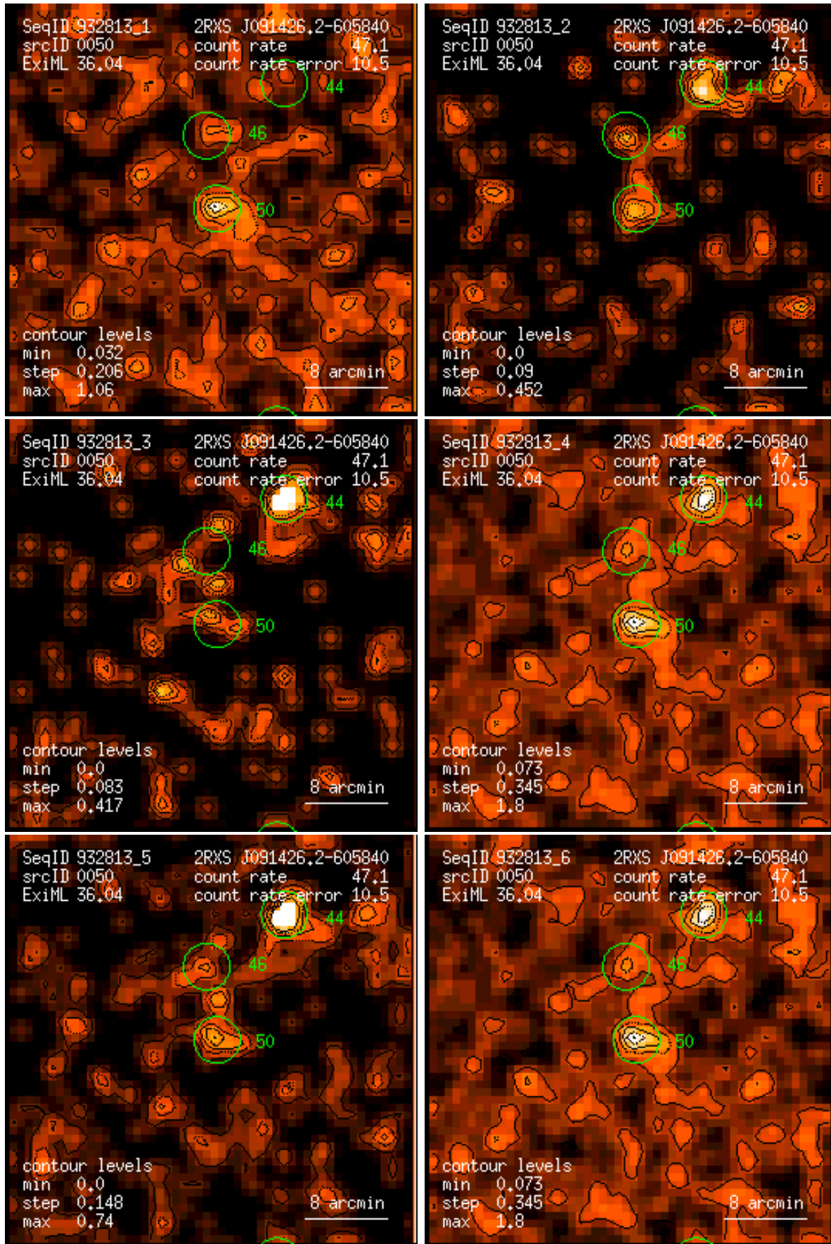
Figure 50: RASS 932813: detection 0050: band rate images, Gaussian filter: (1) PSPC channels 11 – 41, (2) 52 – 90, (3) 91 – 201, (4) 11 – 235, (5) 52 – 201, (6) 11 – 201. Broad band rates in counts/ks. Band rate contour levels in counts/ks/arcmin 2 .
