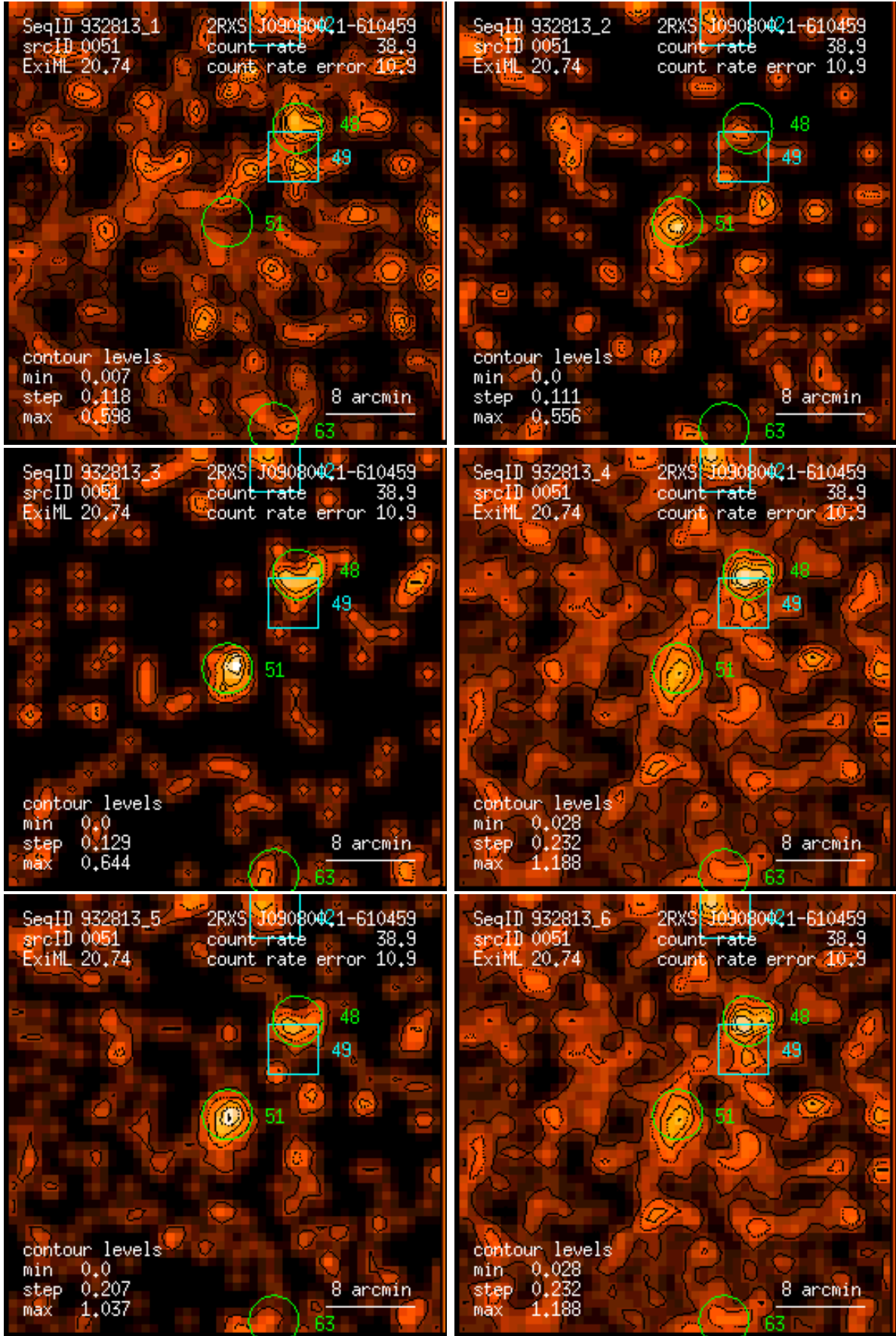
Figure 51: RASS 932813: detection 0051: band rate images, Gaussian filter: (1) PSPC channels 11 – 41, (2) 52 – 90, (3) 91 – 201, (4) 11 – 235, (5) 52 – 201, (6) 11 – 201. Broad band rates in counts/ks. Band rate contour levels in counts/ks/arcmin 2 .
