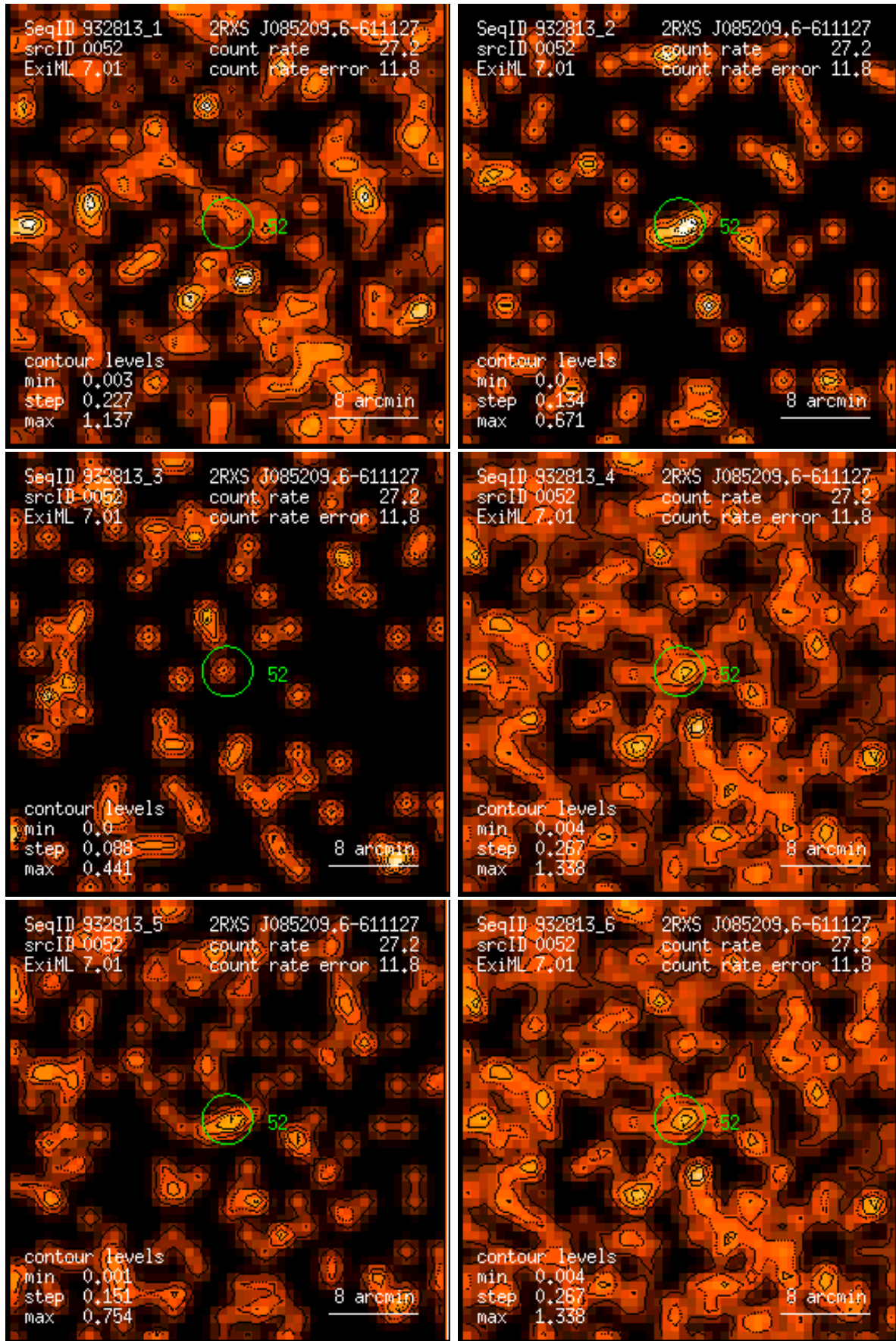
Figure 52: RASS 932813: detection 0052: band rate images, Gaussian filter: (1) PSPC channels 11 – 41, (2) 52 – 90, (3) 91 – 201, (4) 11 – 235, (5) 52 – 201, (6) 11 – 201. Broad band rates in counts/ks. Band rate contour levels in counts/ks/arcmin 2 .
