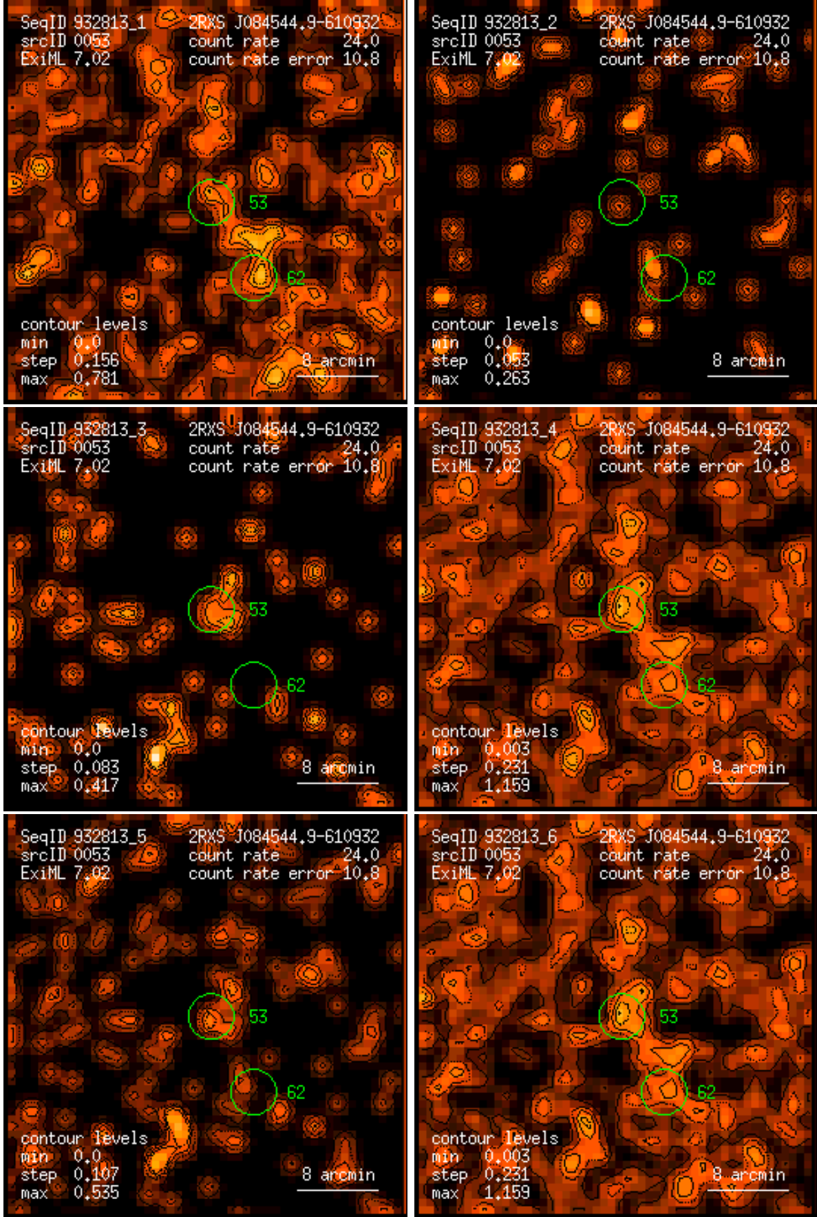
Figure 53: RASS 932813: detection 0053: band rate images, Gaussian filter: (1) PSPC channels 11 – 41, (2) 52 – 90, (3) 91 – 201, (4) 11 – 235, (5) 52 – 201, (6) 11 – 201. Broad band rates in counts/ks. Band rate contour levels in counts/ks/arcmin 2 .
