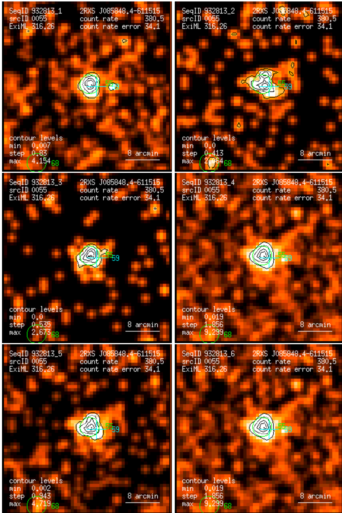
Figure 55: RASS 932813: detection 0055: band rate images, Gaussian filter: (1) PSPC channels 11 – 41, (2) 52 – 90, (3) 91 – 201, (4) 11 – 235, (5) 52 – 201, (6) 11 – 201. Broad band rates in counts/ks. Band rate contour levels in counts/ks/arcmin 2 .
