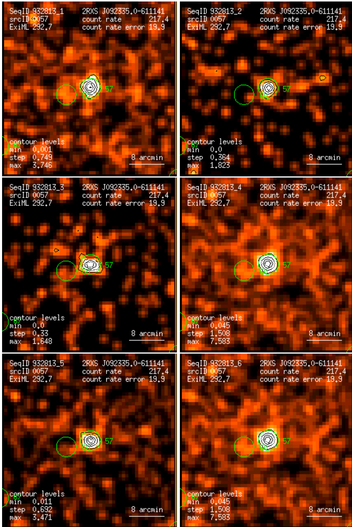
Figure 57: RASS 932813: detection 0057: band rate images, Gaussian filter: (1) PSPC channels 11 – 41, (2) 52 – 90, (3) 91 – 201, (4) 11 – 235, (5) 52 – 201, (6) 11 – 201. Broad band rates in counts/ks. Band rate contour levels in counts/ks/arcmin 2 .
