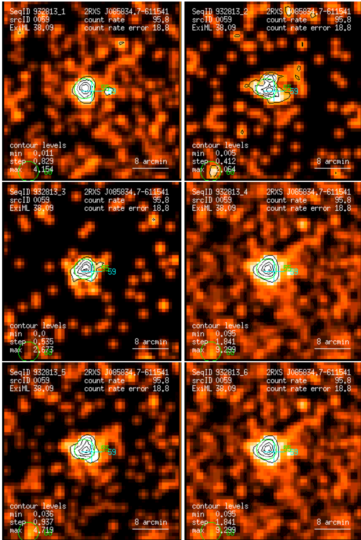
Figure 59: RASS 932813: detection 0059: band rate images, Gaussian filter: (1) PSPC channels 11 – 41, (2) 52 – 90, (3) 91 – 201, (4) 11 – 235, (5) 52 – 201, (6) 11 – 201. Broad band rates in counts/ks. Band rate contour levels in counts/ks/arcmin 2 .
