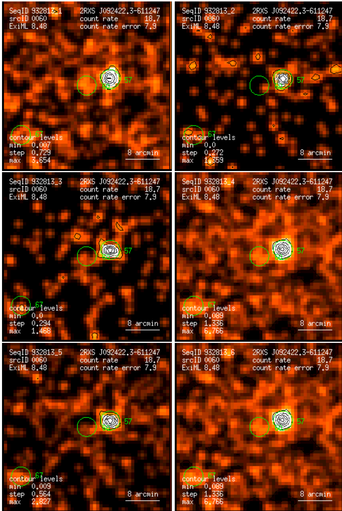
Figure 60: RASS 932813: detection 0060: band rate images, Gaussian filter: (1) PSPC channels 11 – 41, (2) 52 – 90, (3) 91 – 201, (4) 11 – 235, (5) 52 – 201, (6) 11 – 201. Broad band rates in counts/ks. Band rate contour levels in counts/ks/arcmin 2 .
