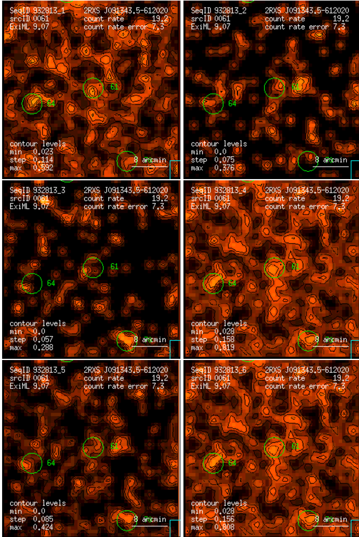
Figure 61: RASS 932813: detection 0061: band rate images, Gaussian filter: (1) PSPC channels 11 – 41, (2) 52 – 90, (3) 91 – 201, (4) 11 – 235, (5) 52 – 201, (6) 11 – 201. Broad band rates in counts/ks. Band rate contour levels in counts/ks/arcmin 2 .
