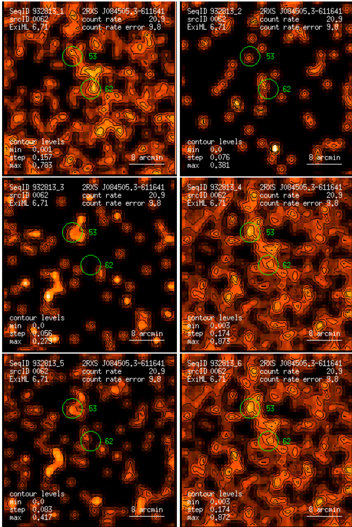
Figure 62: RASS 932813: detection 0062: band rate images, Gaussian filter: (1) PSPC channels 11 – 41, (2) 52 – 90, (3) 91 – 201, (4) 11 – 235, (5) 52 – 201, (6) 11 – 201. Broad band rates in counts/ks. Band rate contour levels in counts/ks/arcmin 2 .
