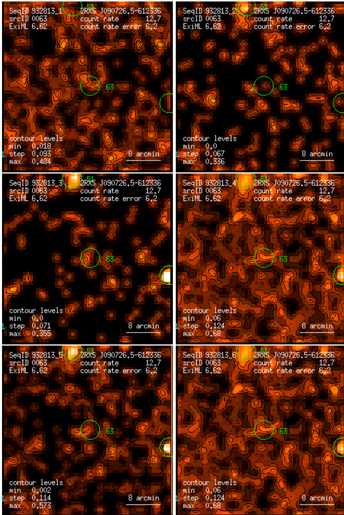
Figure 63: RASS 932813: detection 0063: band rate images, Gaussian filter: (1) PSPC channels 11 – 41, (2) 52 – 90, (3) 91 – 201, (4) 11 – 235, (5) 52 – 201, (6) 11 – 201. Broad band rates in counts/ks. Band rate contour levels in counts/ks/arcmin 2 .
