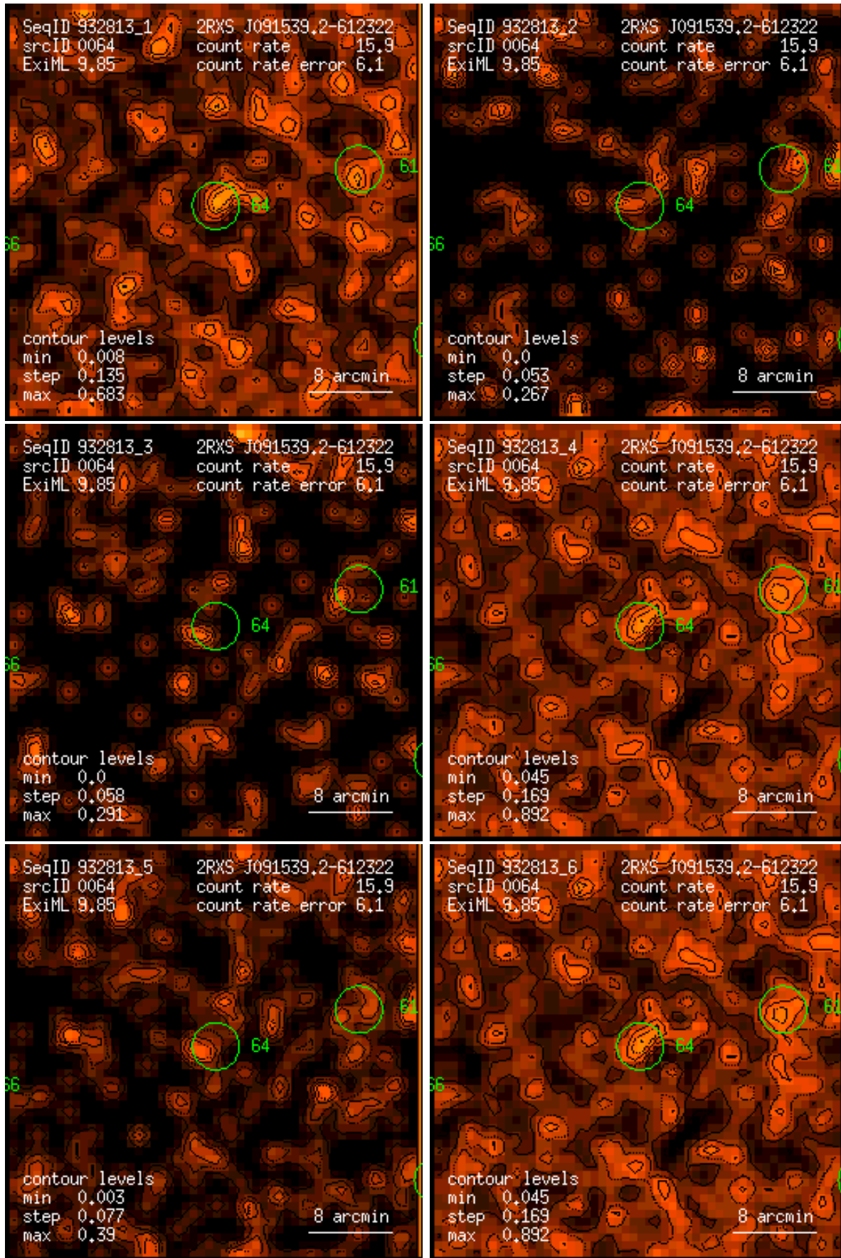
Figure 64: RASS 932813: detection 0064: band rate images, Gaussian filter: (1) PSPC channels 11 – 41, (2) 52 – 90, (3) 91 – 201, (4) 11 – 235, (5) 52 – 201, (6) 11 – 201. Broad band rates in counts/ks. Band rate contour levels in counts/ks/arcmin 2 .
