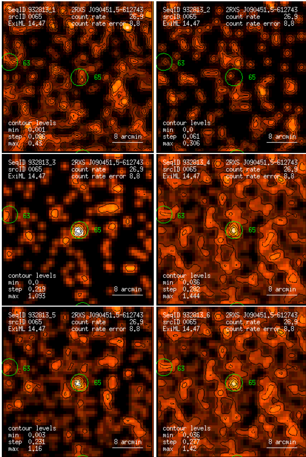
Figure 65: RASS 932813: detection 0065: band rate images, Gaussian filter: (1) PSPC channels 11 – 41, (2) 52 – 90, (3) 91 – 201, (4) 11 – 235, (5) 52 – 201, (6) 11 – 201. Broad band rates in counts/ks. Band rate contour levels in counts/ks/arcmin 2 .
