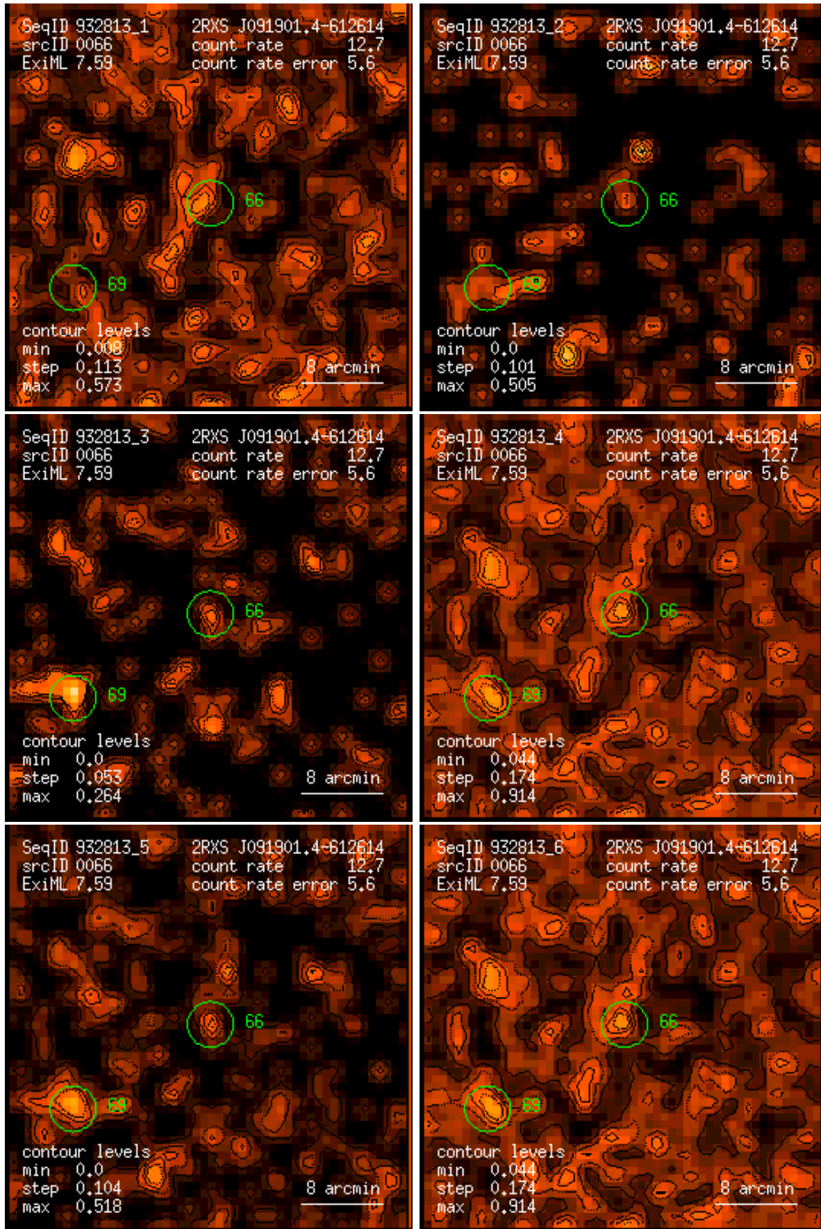
Figure 66: RASS 932813: detection 0066: band rate images, Gaussian filter: (1) PSPC channels 11 – 41, (2) 52 – 90, (3) 91 – 201, (4) 11 – 235, (5) 52 – 201, (6) 11 – 201. Broad band rates in counts/ks. Band rate contour levels in counts/ks/arcmin 2 .
