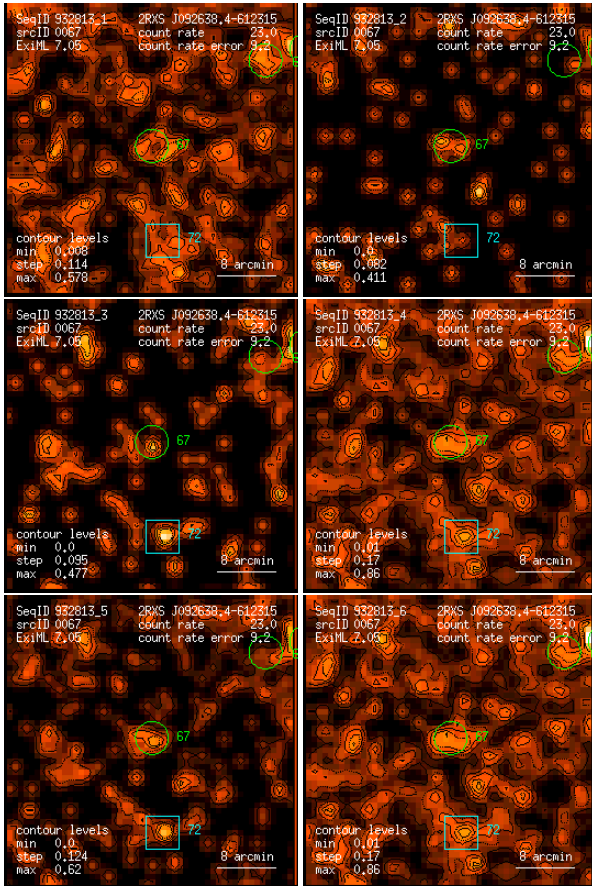
Figure 67: RASS 932813: detection 0067: band rate images, Gaussian filter: (1) PSPC channels 11 – 41, (2) 52 – 90, (3) 91 – 201, (4) 11 – 235, (5) 52 – 201, (6) 11 – 201. Broad band rates in counts/ks. Band rate contour levels in counts/ks/arcmin 2 .
