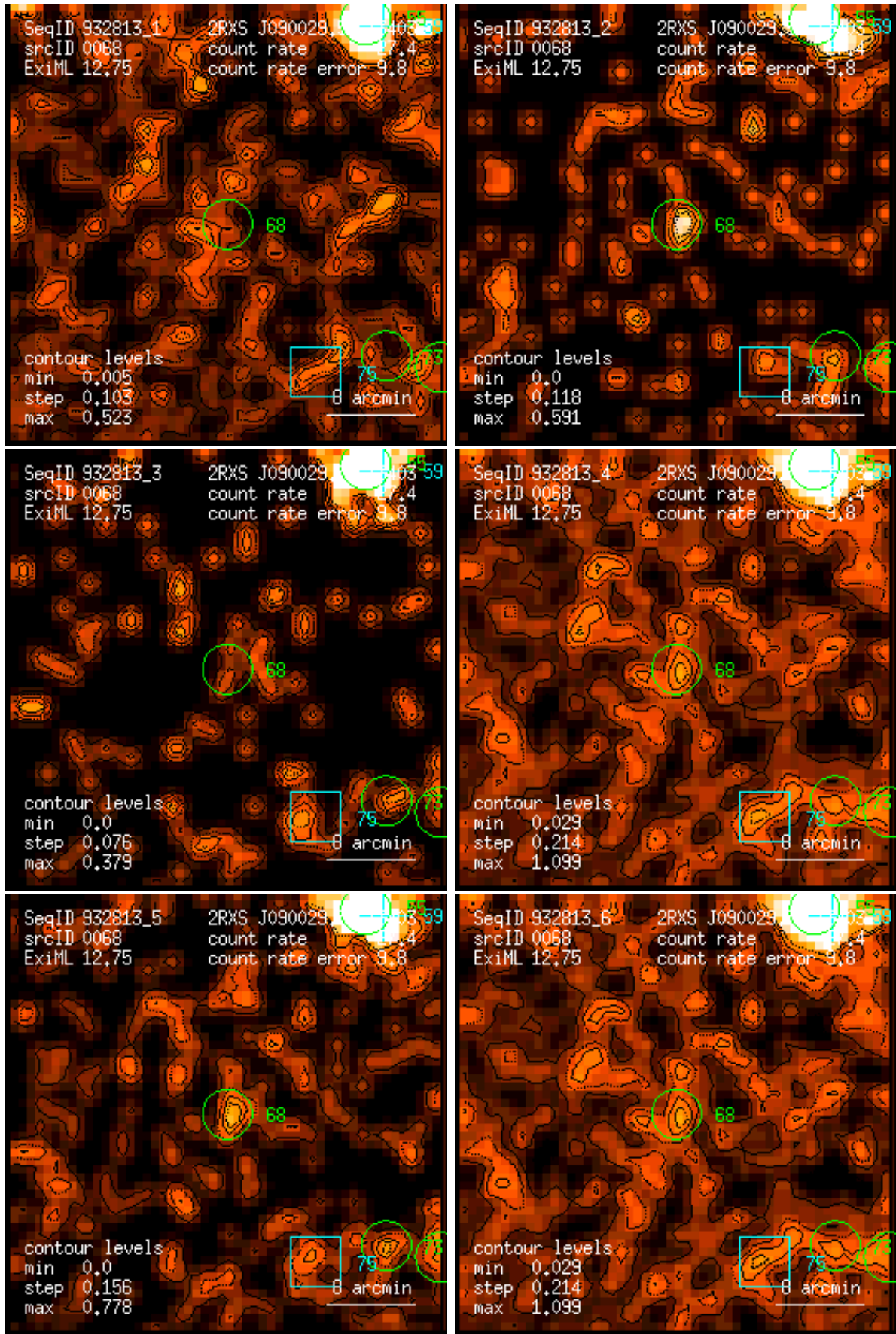
Figure 68: RASS 932813: detection 0068: band rate images, Gaussian filter: (1) PSPC channels 11 – 41, (2) 52 – 90, (3) 91 – 201, (4) 11 – 235, (5) 52 – 201, (6) 11 – 201. Broad band rates in counts/ks. Band rate contour levels in counts/ks/arcmin 2 .
