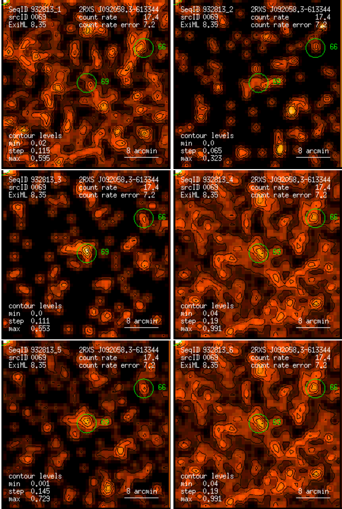
Figure 69: RASS 932813: detection 0069: band rate images, Gaussian filter: (1) PSPC channels 11 – 41, (2) 52 – 90, (3) 91 – 201, (4) 11 – 235, (5) 52 – 201, (6) 11 – 201. Broad band rates in counts/ks. Band rate contour levels in counts/ks/arcmin 2 .
