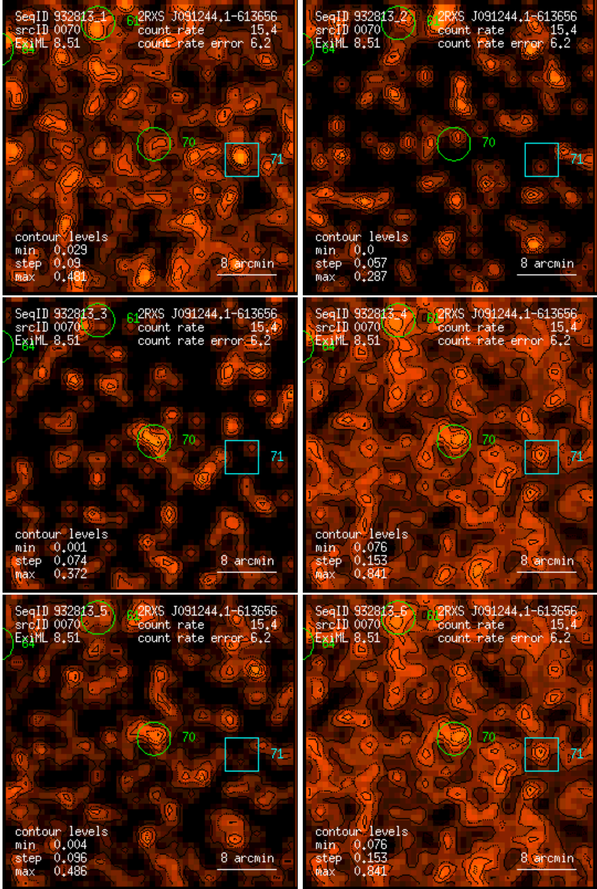
Figure 70: RASS 932813: detection 0070: band rate images, Gaussian filter: (1) PSPC channels 11 – 41, (2) 52 – 90, (3) 91 – 201, (4) 11 – 235, (5) 52 – 201, (6) 11 – 201. Broad band rates in counts/ks. Band rate contour levels in counts/ks/arcmin 2 .
