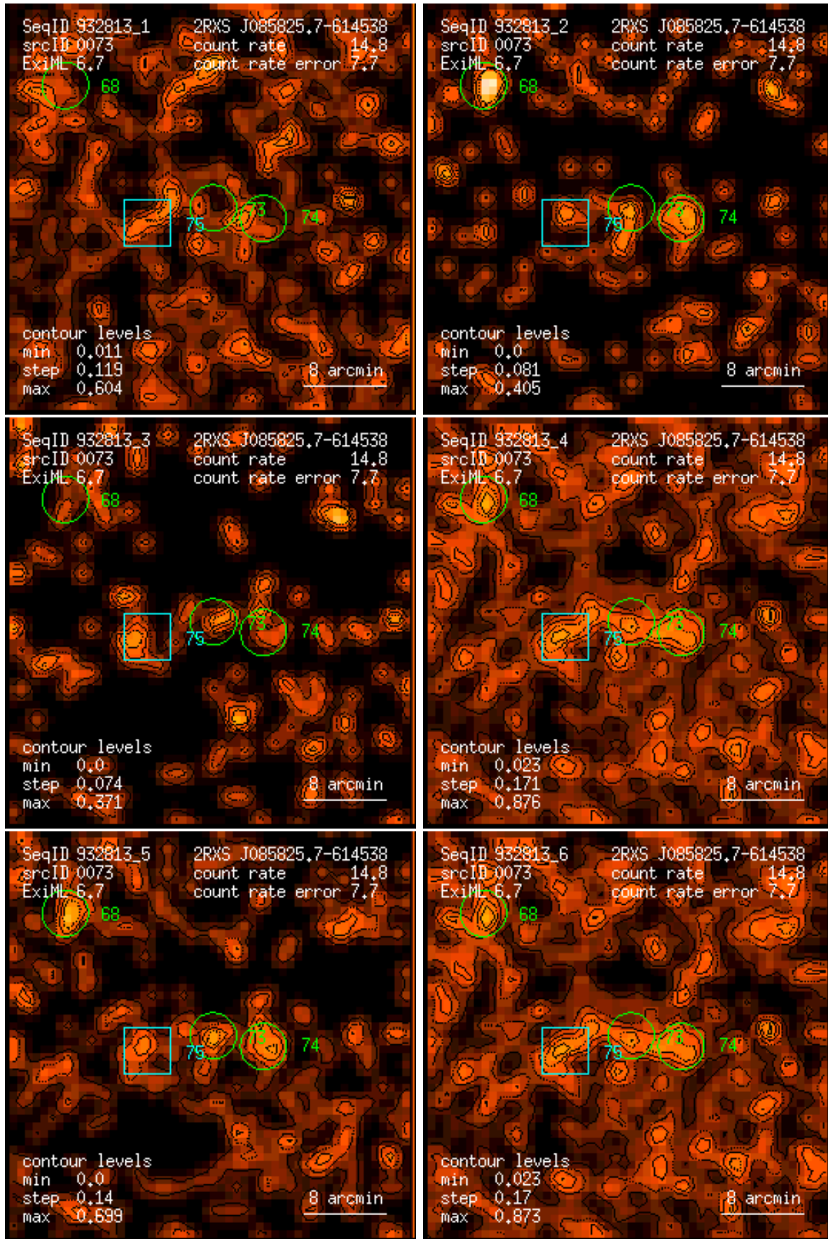
Figure 73: RASS 932813: detection 0073: band rate images, Gaussian filter: (1) PSPC channels 11 – 41, (2) 52 – 90, (3) 91 – 201, (4) 11 – 235, (5) 52 – 201, (6) 11 – 201. Broad band rates in counts/ks. Band rate contour levels in counts/ks/arcmin 2 .
