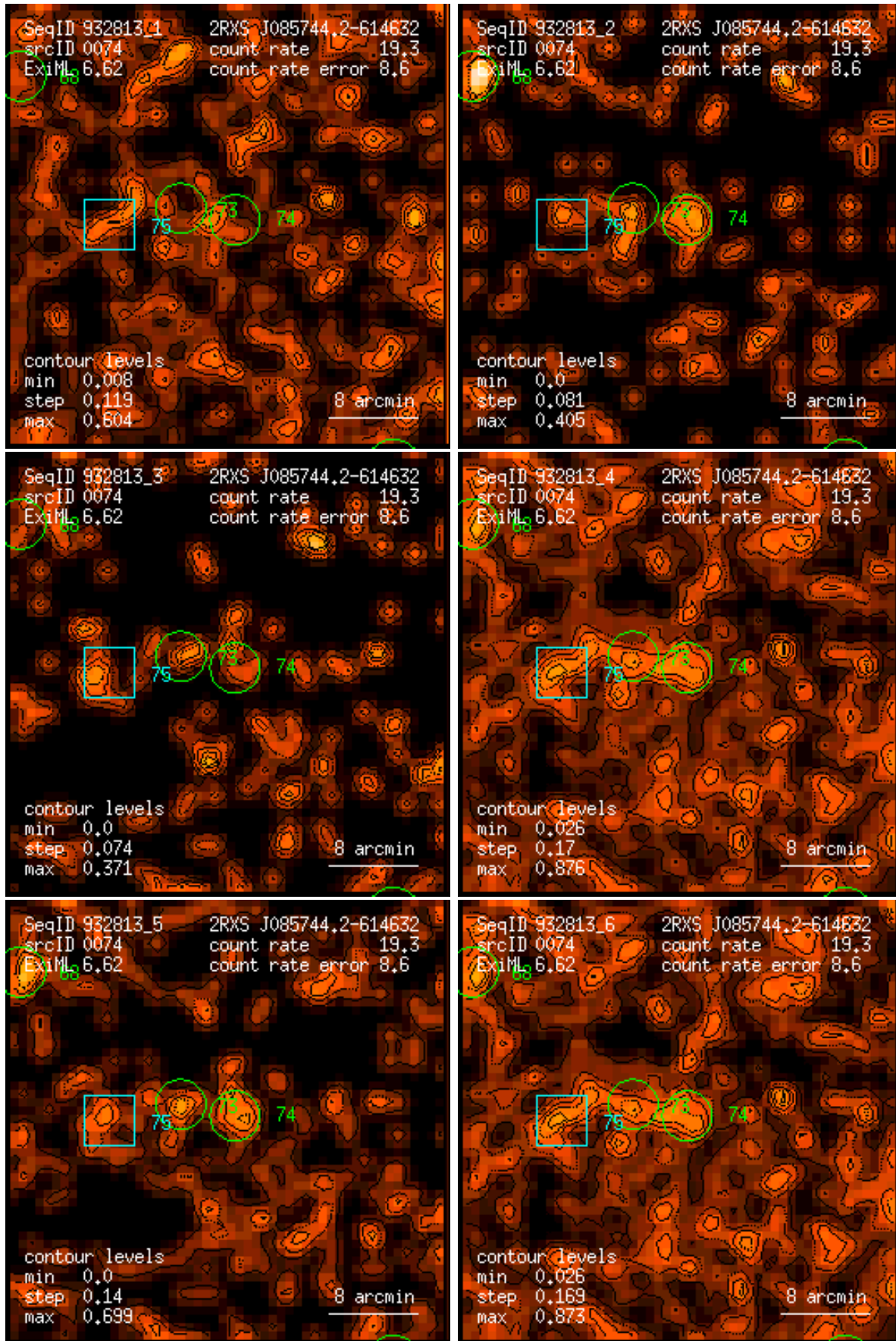
Figure 74: RASS 932813: detection 0074: band rate images, Gaussian filter: (1) PSPC channels 11 – 41, (2) 52 – 90, (3) 91 – 201, (4) 11 – 235, (5) 52 – 201, (6) 11 – 201. Broad band rates in counts/ks. Band rate contour levels in counts/ks/arcmin 2 .
