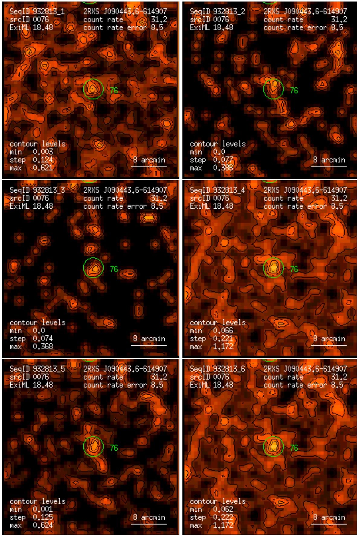
Figure 76: RASS 932813: detection 0076: band rate images, Gaussian filter: (1) PSPC channels 11 – 41, (2) 52 – 90, (3) 91 – 201, (4) 11 – 235, (5) 52 – 201, (6) 11 – 201. Broad band rates in counts/ks. Band rate contour levels in counts/ks/arcmin 2 .
