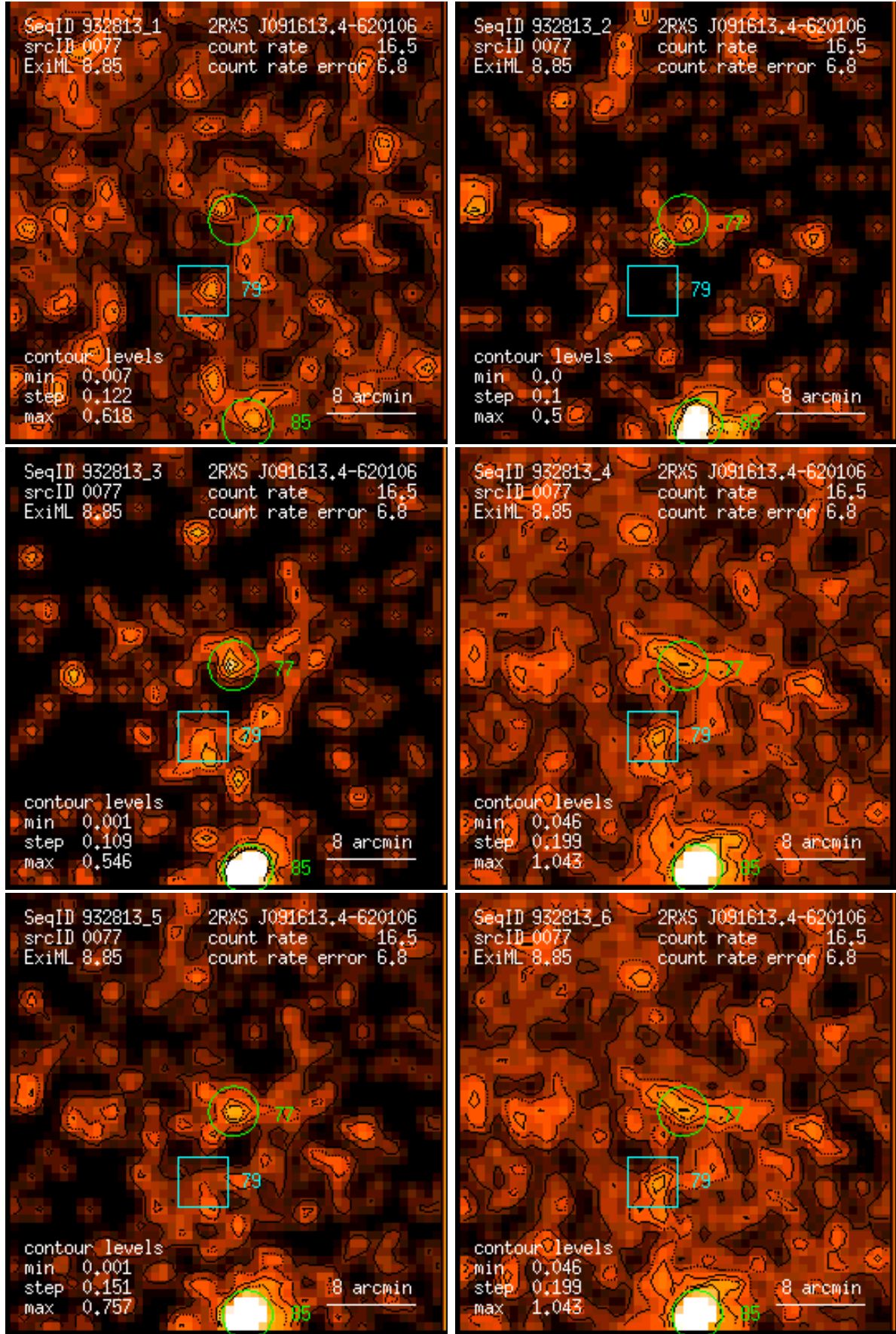
Figure 77: RASS 932813: detection 0077: band rate images, Gaussian filter: (1) PSPC channels 11 – 41, (2) 52 – 90, (3) 91 – 201, (4) 11 – 235, (5) 52 – 201, (6) 11 – 201. Broad band rates in counts/ks. Band rate contour levels in counts/ks/arcmin 2 .
