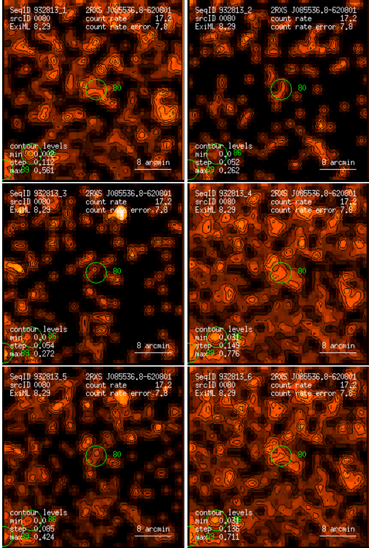
Figure 80: RASS 932813: detection 0080: band rate images, Gaussian filter: (1) PSPC channels 11 – 41, (2) 52 – 90, (3) 91 – 201, (4) 11 – 235, (5) 52 – 201, (6) 11 – 201. Broad band rates in counts/ks. Band rate contour levels in counts/ks/arcmin 2 .
