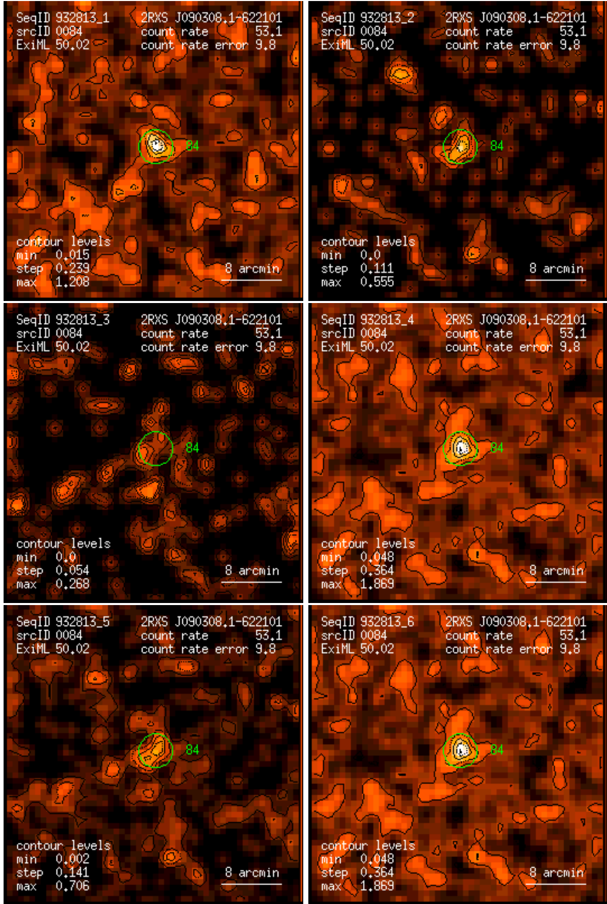
Figure 84: RASS 932813: detection 0084: band rate images, Gaussian filter: (1) PSPC channels 11 – 41, (2) 52 – 90, (3) 91 – 201, (4) 11 – 235, (5) 52 – 201, (6) 11 – 201. Broad band rates in counts/ks. Band rate contour levels in counts/ks/arcmin 2 .
